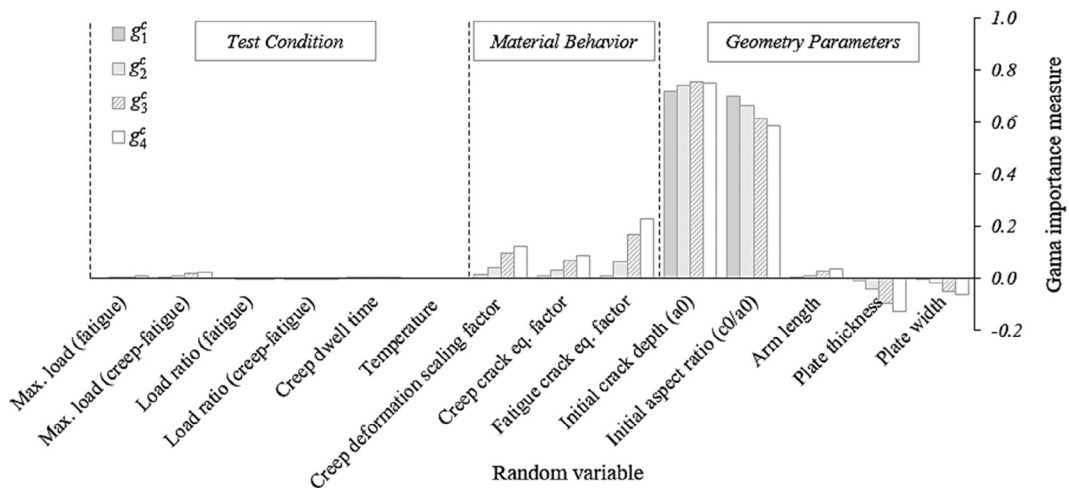
Fig. 13. \gamma importance measure associated to crack surface limit state functions, g_i^c(\mathbf{x}) .
