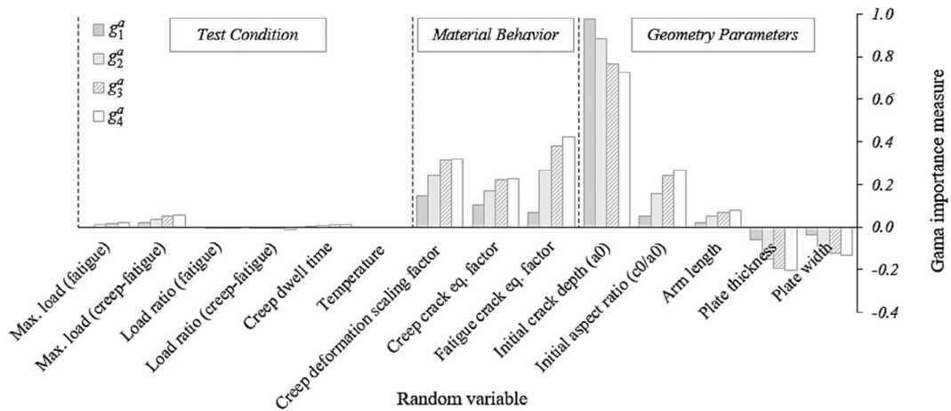
Fig. 12. \gamma importance measure associated to crack depth limit state functions, g_i^a(\mathbf{x}) .
