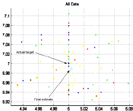
Figure IV-7 Three sensor, single target estimate data
