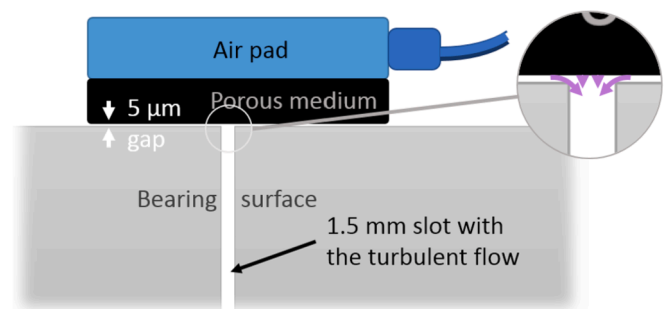
Fig. 3. Schematic side view of the air pad. The air is expelled by the porous media into the 5 \mu\text{m} gap between the air pad and the bearing surface. During the 'slot-passing', some air will be expelled into this channel from the porous media and from the air gap.
