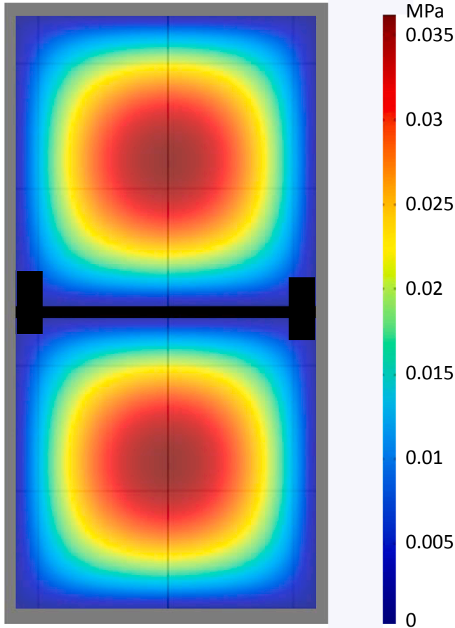
Fig. 4. Simulation result illustrating the behaviour of the air pressure under the porous media of the pad. A similar reduction in pressure is observed at the edge of the pad (grey line) and at the edge of the bearing surface (black line).
