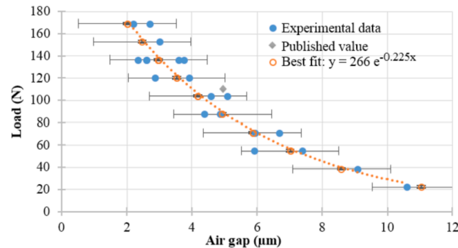
Fig. 10. Lift/Load curve obtained from the 20 mm × 40 mm porous air bearing. The error bars demonstrate the uncertainty of each of the best fit values, which have 99.7% confidence intervals of \pm 1 N and \pm 1.1 μm, for the load and air gap, respectively.
