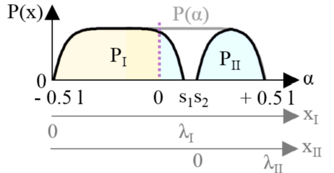
Fig. 7. The pressure distributions P_I and P_{II} are identified. The integral P_I is shown in light yellow and P_2 in light blue, on each side of the pad's middle (shown as a purple dashed line).
