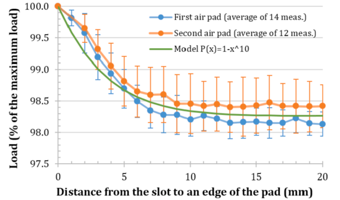
Fig. 12. Static load of a 20 mm × 40 mm air pad as a function of the position of a 1.5 mm large slot sliding below the pad, along its length. The results are expressed as percentages of the maximum load and the errors bars show the 67% confidence intervals.
