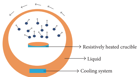
FIGURE 7: Preparation of nanofluid using one-step vapour deposition method [23].
