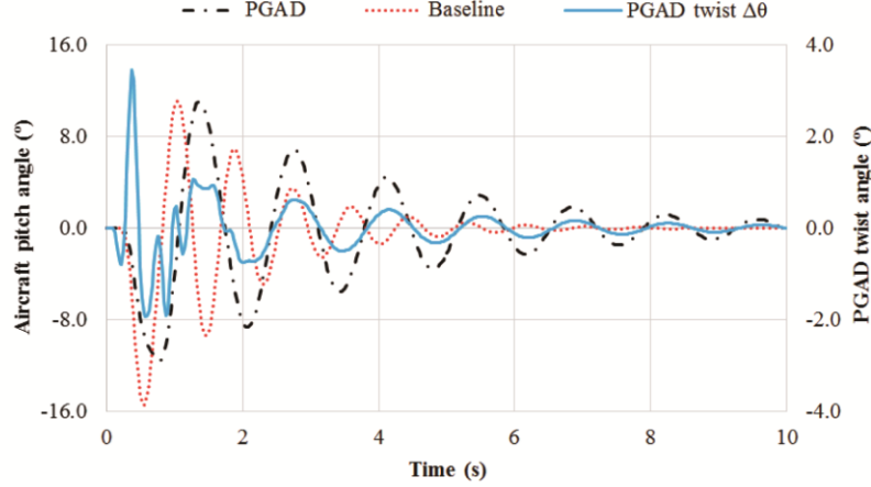
Figure 17. The aircraft pitching angle and PGAD twist angle in response to the gust
