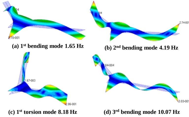
Figure 5. The first four symmetric mode shapes of the flying-wing structure
