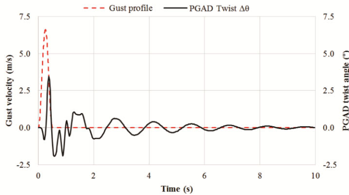
Figure 14. Gust velocity and corresponding PGAD twist angle
