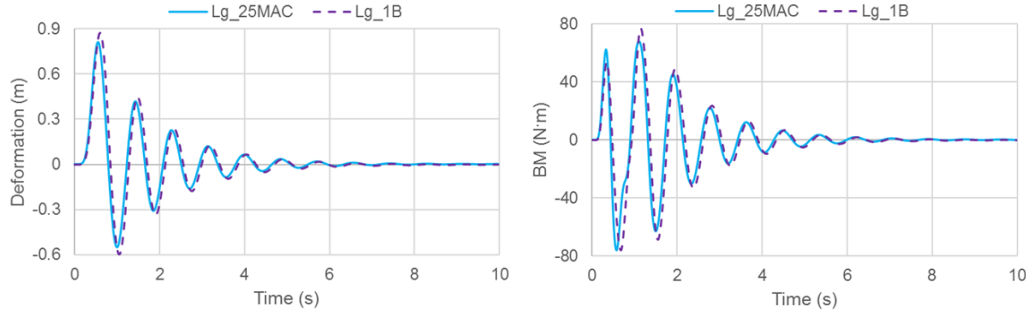
Figure 8. (a) The wing deflection and (b) bending moment in response to the typical gust ( L_g\_25\text{MAC} ) and the gust of the wing 1 st bending frequency ( L_g\_1\text{B} )
