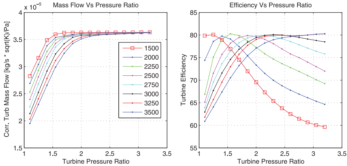
Fig. 3 Turbine map for the AMT Olympus engine
