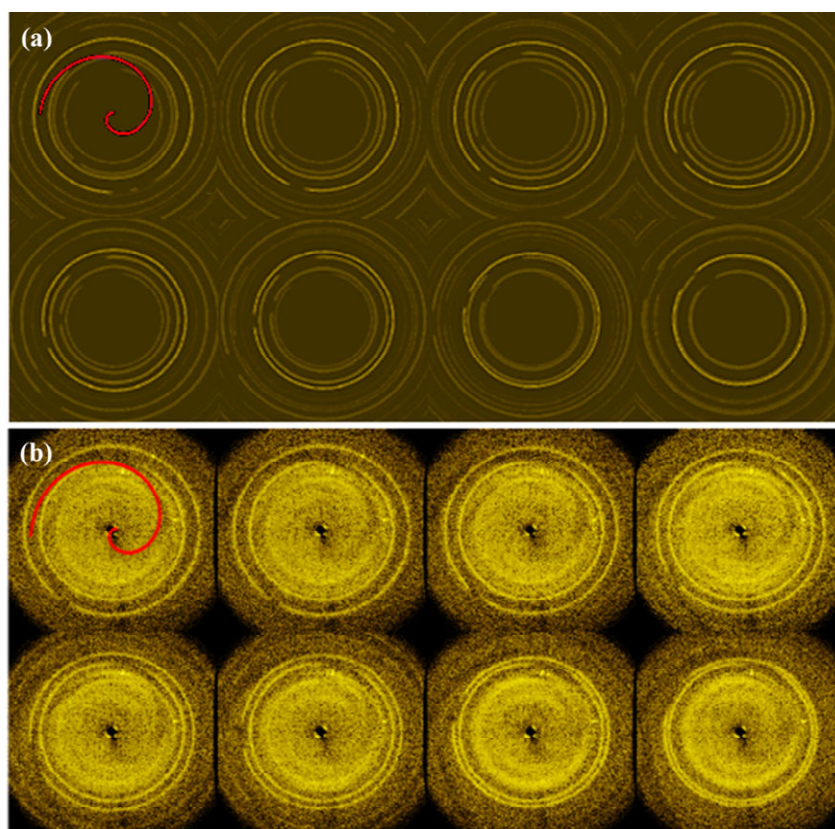
Figure 9 (a) A sequence of simulated images and (b) a sequence of diffraction patterns from a pair of calcite samples spatially separated along the primary axis with a spiral encoder in front of the detector. The sequence was recorded as one of the samples was translated towards the detector face.
