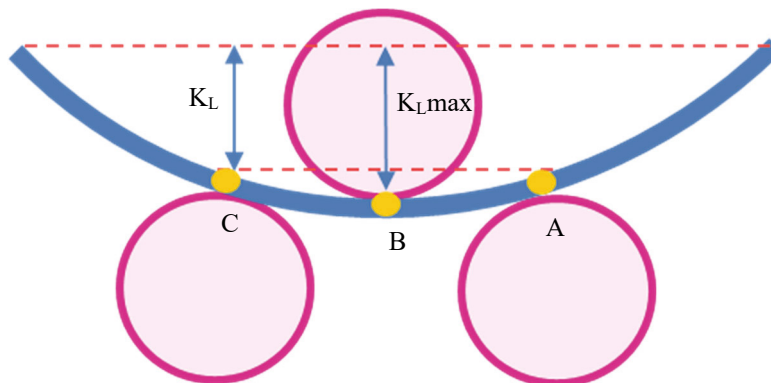
Figure 1 – Schematic of three roll bending process
