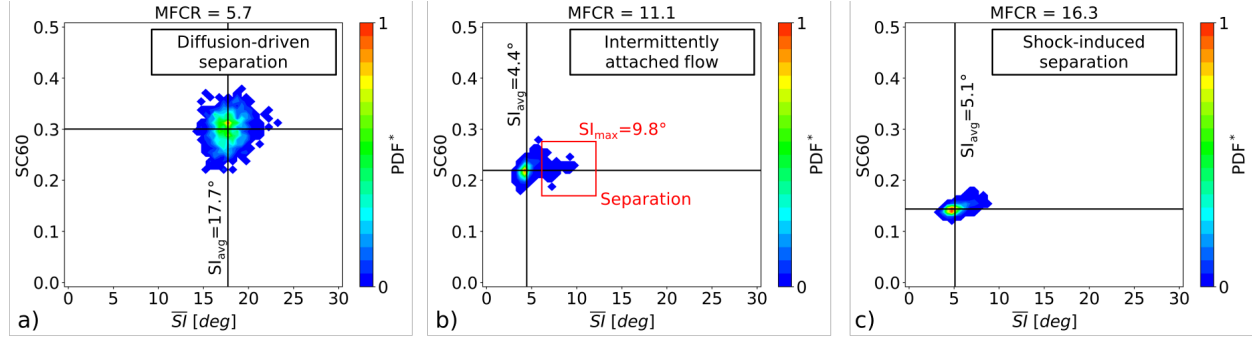
Figure 10 SC60-\overline{SI} j-PDF distributions at the AIP: a) MFCR = 5.7 ; b) MFCR = 11.1 ; c) MFCR = 16.3 for a fixed crosswind velocity of 15 kts (7.7 m/s).
