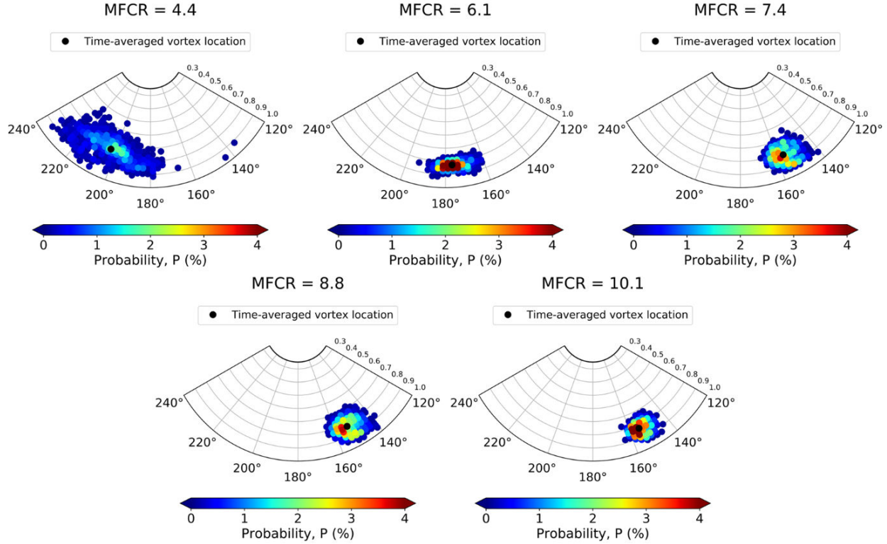
Figure 9 Distribution of instantaneous ground vortex locations at the AIP as a function of Mass Flow Capture Ratio ( MFCR ) for a fixed crosswind velocity of 20 kts (10.3 m/s).
