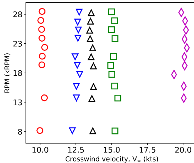
Figure 15 Operating conditions tested during the crosswind campaign at DNW-LLF.
