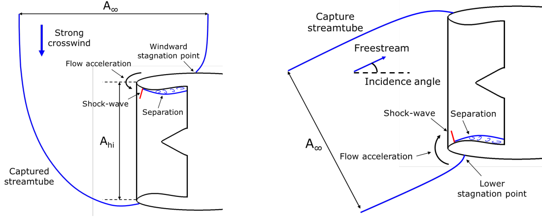
Figure 1 Key flow features within an intake under crosswind (left) and incidence (right) operating conditions.
