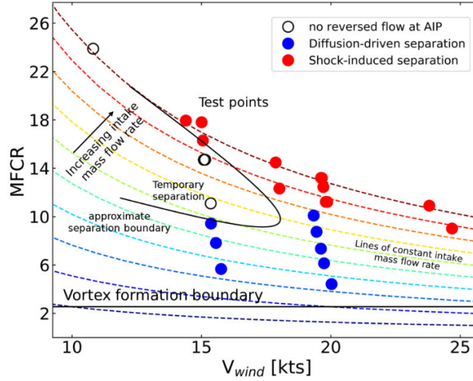
Figure 4 Operating conditions tested during the crosswind campaign at DNW-LST [31].
