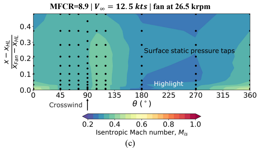
Figure 19 Time-averaged isentropic Mach number distributions across the inner surface of the intake for a constant crosswind velocity of 12.5 kts and MFCR=17.5 and MFCR=8.9.
