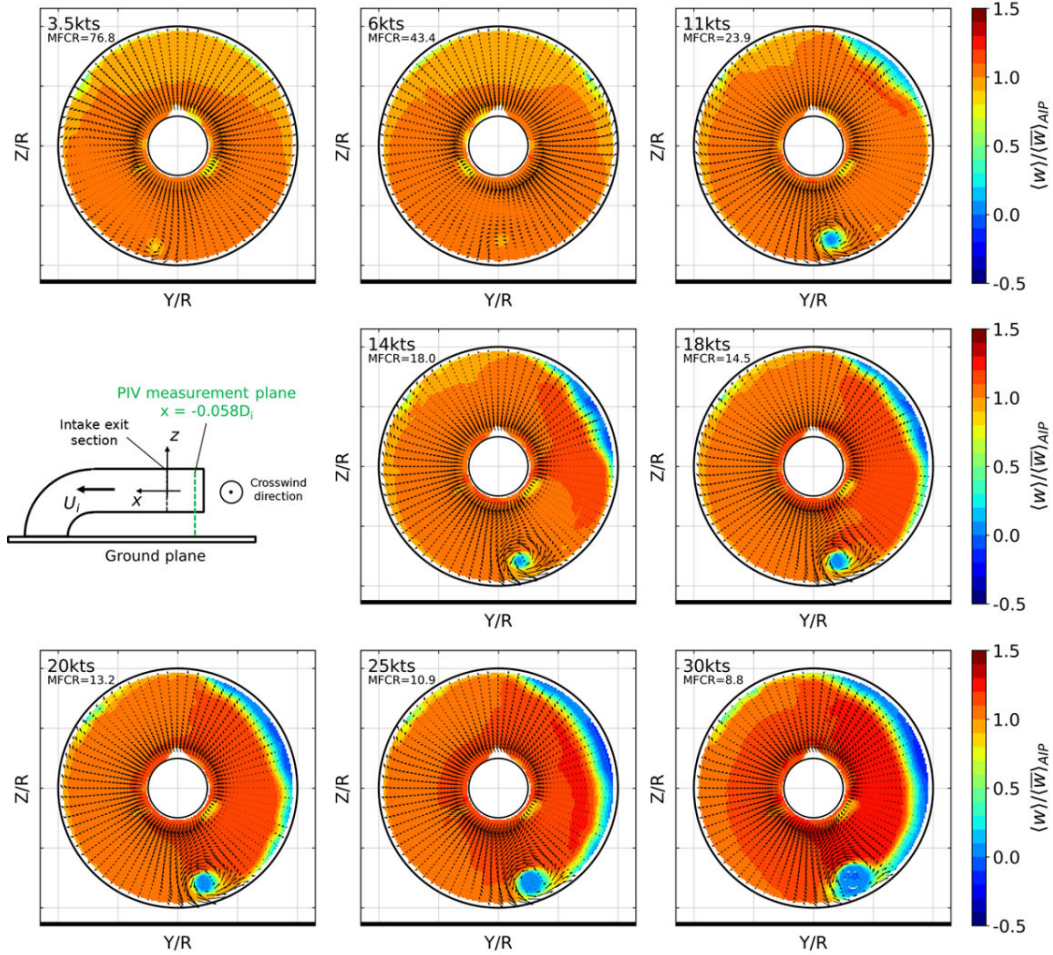
Figure 6 PIV measured time-averaged normalized axial velocity at the AIP with crosswind velocity for a fixed maximum intake mass flow rate. Crosswind direction from right to left. View looking downstream.
