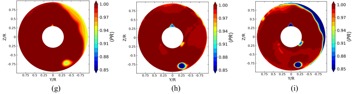
Figure 11 Measured and reconstructed time-averaged total pressure ratio distributions for the case at 15 kts (7.7 m/s). View looking downstream.
