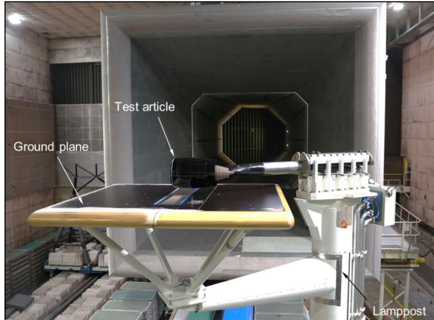
Figure 12 Test article and ground plane installed at DNW-LLF open working section via a lamppost system (view parallel to crosswind direction, looking downstream).
