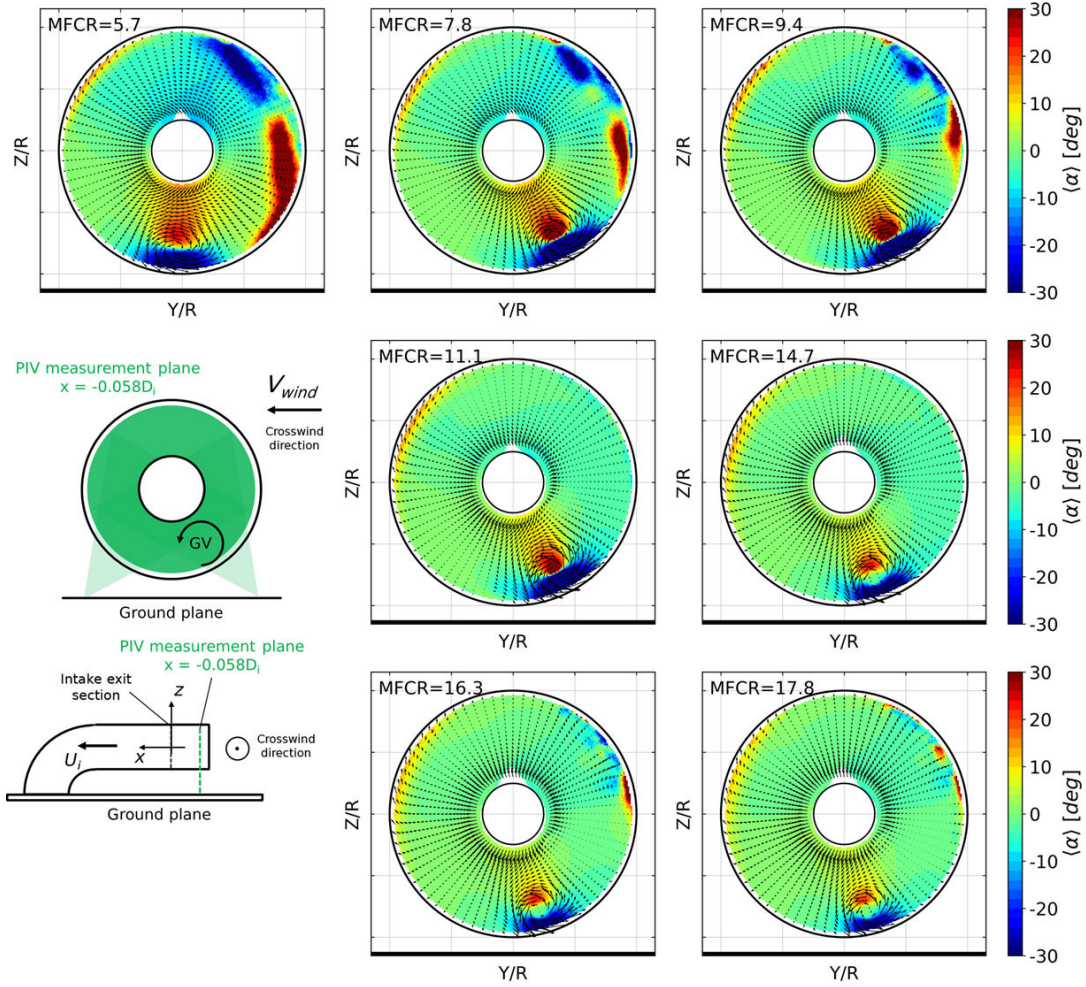
Figure 7 Time-averaged swirl angle distributions at the AIP for increasing Mass Flow Capture Ratio (MFCR) at 15 kts (7.7 m/s). Crosswind direction from right to left. View looking downstream.
