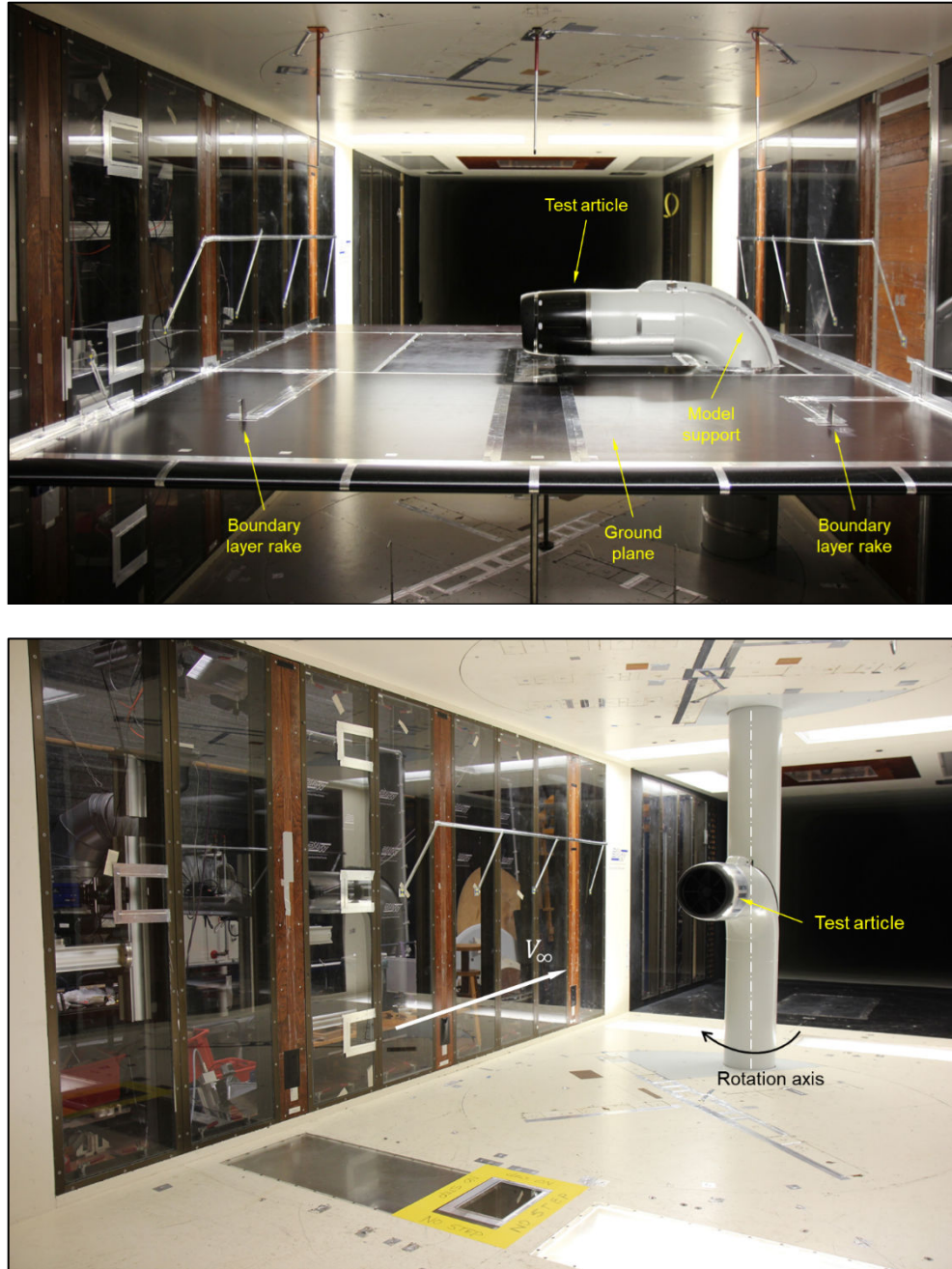
Figure 2 Experimental setups for the crosswind test at DNW-LST. Top: setup for crosswind tests with ground plane. Bottom: setup for angle of attack. Images not to scale [30].
