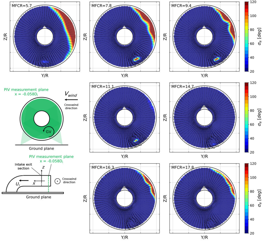
Figure 8 AIP distributions of the swirl angle fluctuations with increasing Mass Flow Capture Ratio (MFCR) for a fixed crosswind velocity of 15 kts (7.7 m/s). Crosswind direction from right to left. View looking downstream.
