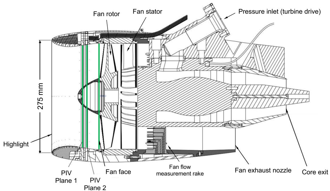
Figure 13 Test article schematic indicating fan face and PIV measurement planes [36].
