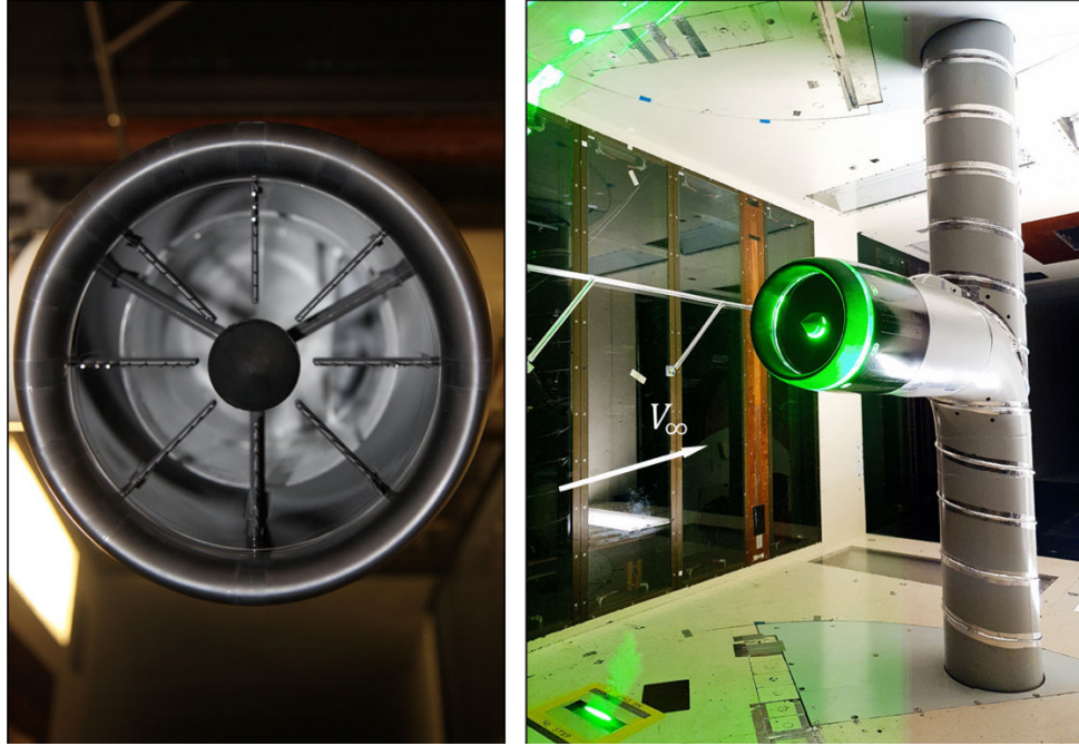
Figure 3 Left: Total pressure rake installed within the test article for total pressure distortion measurement. Right: Test article installed within the DNW-LST at headwind attitude and laser sheet delivered at the notional fan face. Not to scale.
