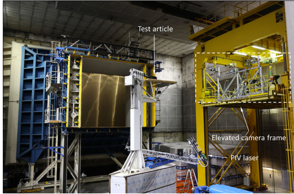
Figure 14 View of the NIFTI-LLF wind tunnel installation indicating the test article in relation to the tunnel's exit nozzle and the location of the PIV camera frame.
