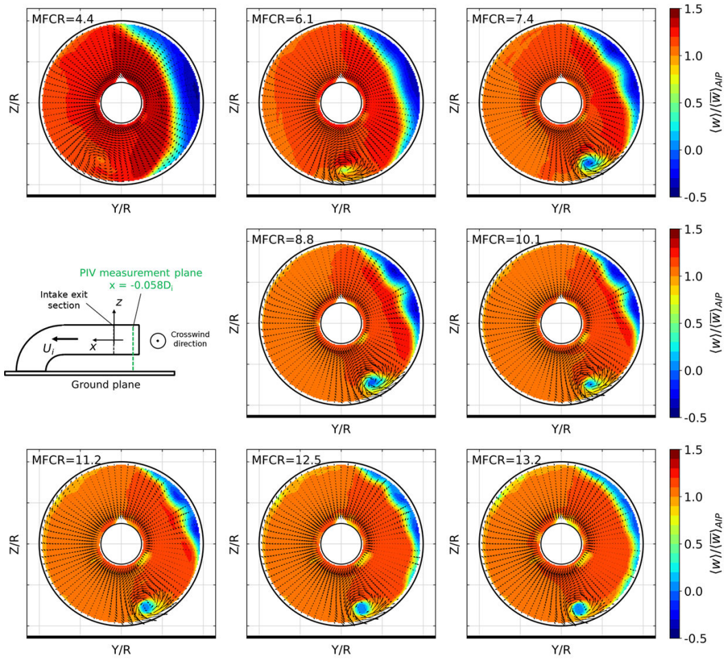
Figure 5 PIV measured time-averaged normalized axial velocity at the AIP with increasing MFCR at a fixed crosswind velocity of 20 kts (10.3 m/s). Crosswind direction from right to left. View looking downstream.
