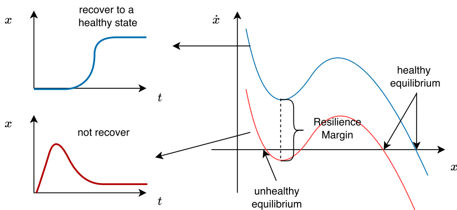
Figure 2. Red line describes a system with more than one stable equilibrium (healthy one and unhealthy one both exist). The system in this situation will remain in a low-level state. The blue line describes a system with only one stable equilibrium, and the system will recover to a high-level state at last. When there exists an unhealthy equilibrium, the system loses resilience. This picture shows the ability of the system to recover to the original state from an undesirable state. The resilience margin shows the ability of the system to withstand the perturbation. If the local minimum value is much larger than 0, the system can withstand more perturbations and keeps resilient. However, if the local minimum value is close to 0, small perturbation may cause the loss of resilience.
