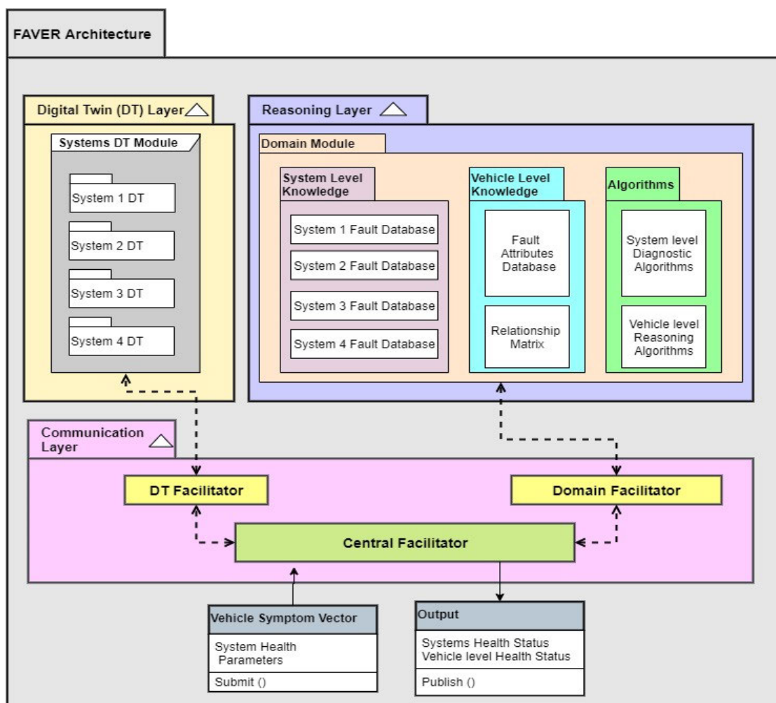
FIGURE 3. The architecture of FAVER.
