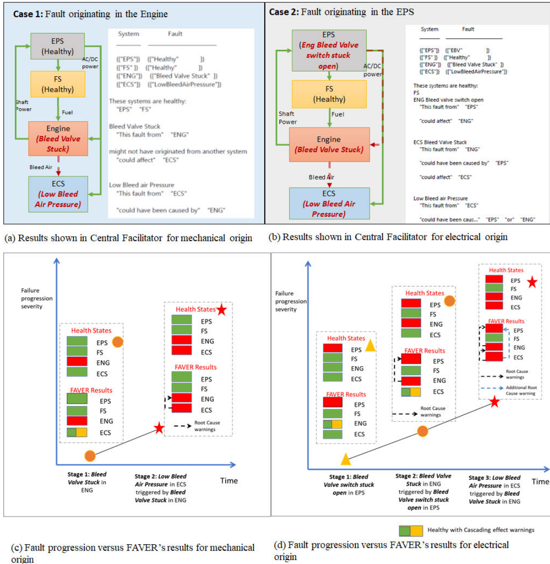
FIGURE 8. Use case scenario of bleed valve stuck fault cascading to the ECS with mechanical and electrical origin.
