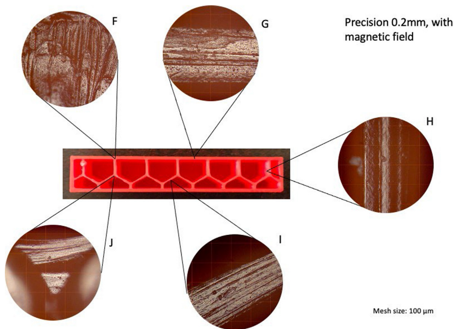
Fig. 9. Printed PLA sample with microscopy - F: Side and boundary, G: Side and hole, H: Straight line, I: Tilted line and J: Intersection.
