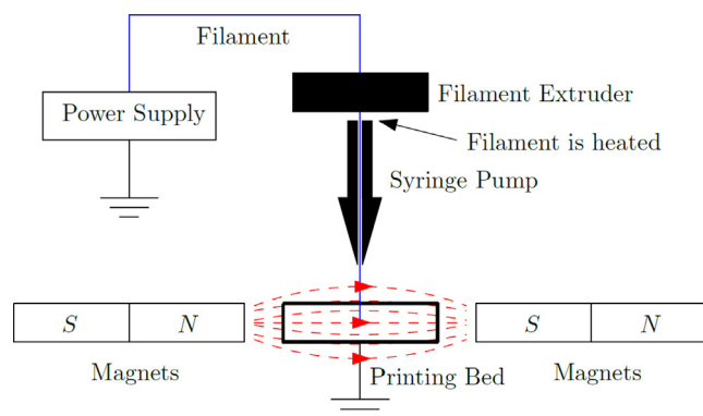
Fig. 1. Diagram of the front view of FDM technique with magnets on either side of the printing bed, where the red dashed line represents the magnetic field going from the north to south pole. (For interpretation of the references to colour in this figure legend, the reader is referred to the web version of this article.)
