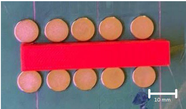
Fig. 4. PLA printed cuboid with five N52 magnets of opposite polarity on each side of the cuboid.
