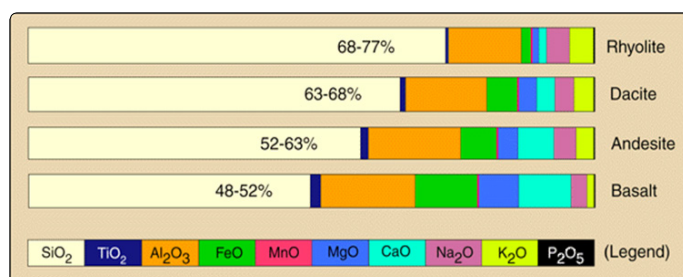
Figure 2. Volcanic Rock Components [4].
