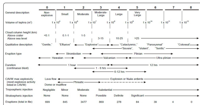
Figure 1. Volcanic Explosivity Index, ICAO [3]
