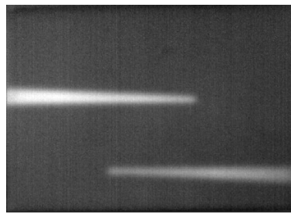
Figure 10. Image composition.
