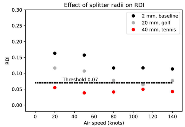
FIGURE 18: RDI VALUES FOR DIFFERENT SPLITTER RADI
