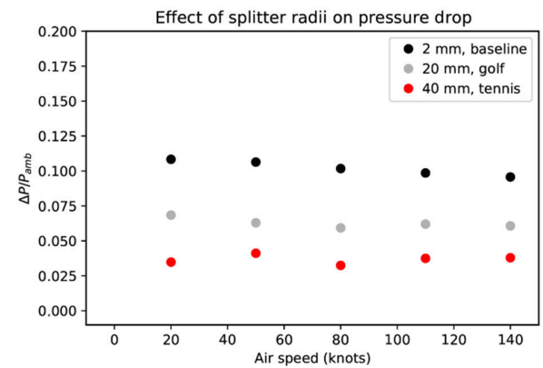
FIGURE 19: REVERSE STREAM PRESSURE LOSS FOR DIFFERENT SPLITTER RADI
