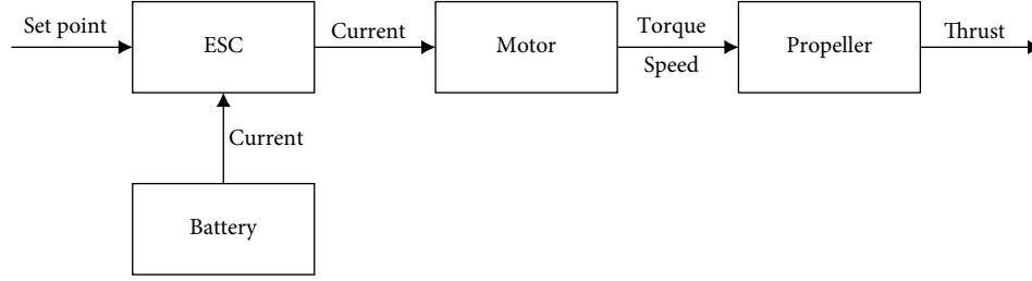
FIGURE 2: Multirotor propulsion chain diagram.
