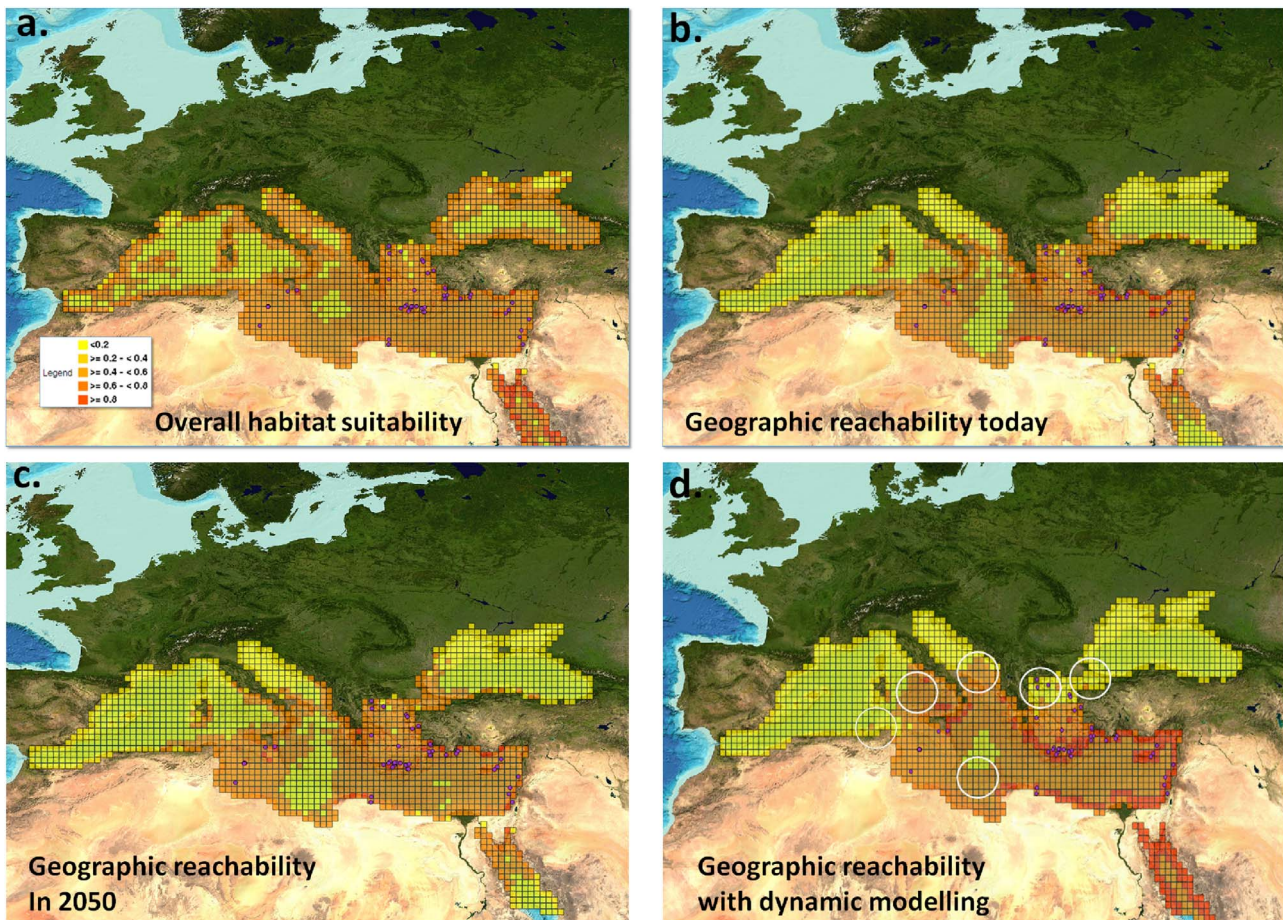
Fig. 4. Comparison between several distributions estimated for L. scleratus in the Mediterranean Sea: (a) overall potential habitat map, obtained by merging the baseline models, (b) geographical reachability distribution calculated by applying a Gaussian spatial weighting operation to the overall potential habitat map, (c) geographical reachability distribution estimated for 2050, and (d) distribution estimated by means of a dynamic model. The overlapping points indicate the real observations of the pufferfish in the Mediterranean Sea that were used to tune the spatial models. The circles in figure (d) indicate the highest discrepancy areas with respect to the distribution in figure (b). The overlaid dark dots represent the observations in the Mediterranean Sea used to train the geographical reachability model. The legend is the same for all the maps.
