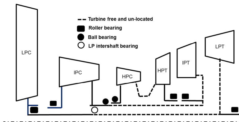
Figure 1 Schematic representation of a three-shaft turbofan engine
