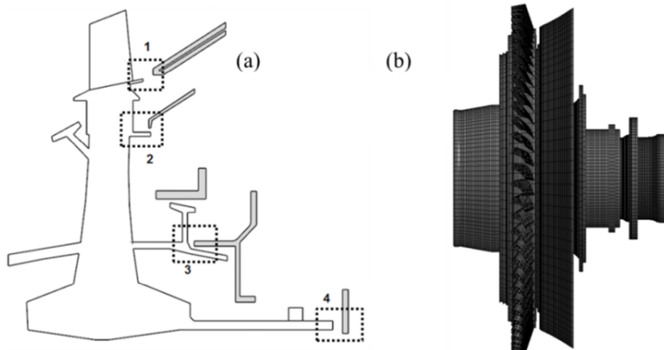
Figure 6 a) Four main contact regions in the turbine assembly b) Front view of the finite element model
