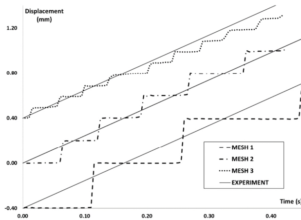
Figure 4 Axial displacement of the left steel bar for the three meshes
