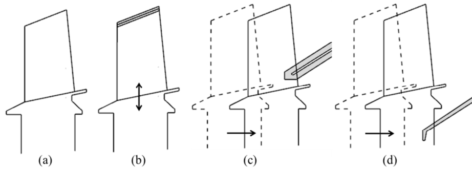
Figure 2 Possible scenarios a) Intact rotor b) Blade shedding c) Blade interference d) Disk rubbing
