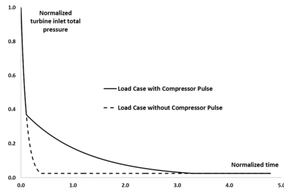
Figure 5 Discharge of gas from upstream combustor reservoir
