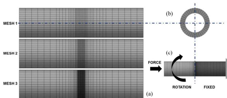
Figure 3 Finite element model of the steel bar friction welding experiment a) Three different meshes from front view b) Side view of all three meshes c) Description of the friction welding
