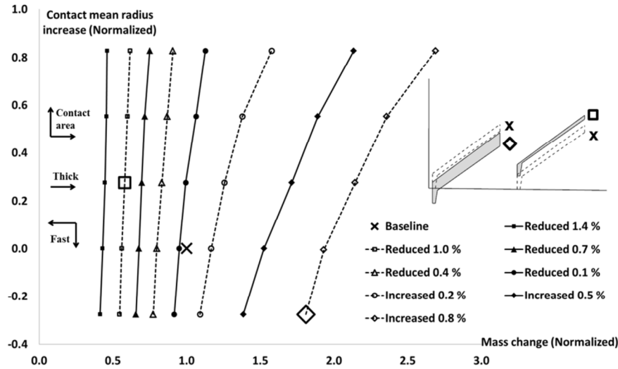
Figure 8 Design space of rotor post shaft failure behaviour by speed iso-lines with sample geometries
