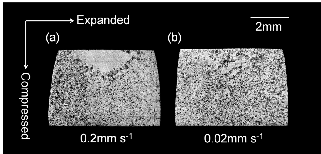
Fig. 7. Optical macrographs of PSC samples compressed at (a) 0.2 \text{ mm s}^{-1} and (b) 0.02 \text{ mm s}^{-1} . Both samples were rapidly heat-treated to 1100 \text{ }^{\circ}\text{C} for 1 s.
