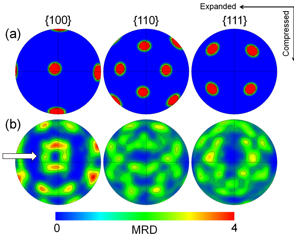
Fig. 6. Pole figures showing the typical ‘before and after’ texture for (a) the unrecrystallized prior parent \beta grain and (b) the RX \beta grains (reconstructed) that formed in the same grain, from a PSC sample, compressed to a height reduction of 14% (sample-centre strain estimated as 20%) under ‘standard’ conditions. Note: the characteristic four-fold motif centred on the parent grains \langle 001 \rangle poles in the \{001\} pole figure for the recrystallized grains in figure (b) (arrow).
