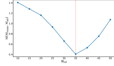
Fig. 5. Distributional Distance between distributional distance between attacked and OOD samples and attacked and adversarial samples for different refinement iterations
