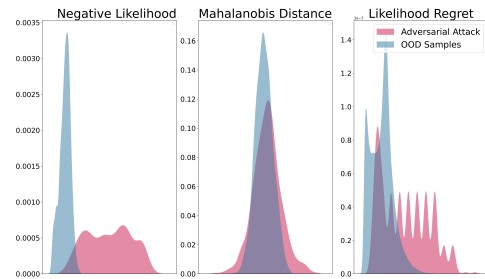
Fig. 6. The metrics to detect adversarial samples from OOD samples (a) NLL (b) Mahalanobis Distance (c) Likelihood regret.
