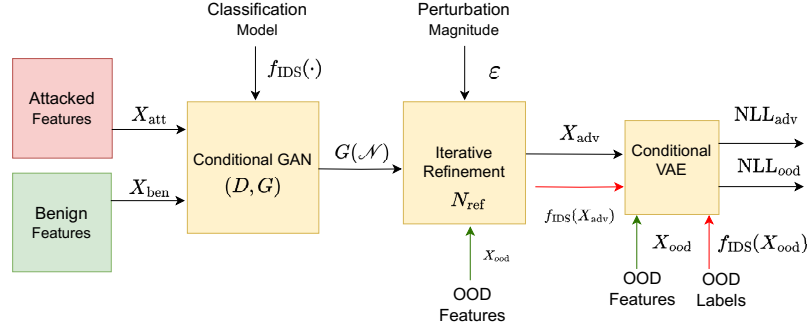
Fig. 2. Schematic for obtaining negative likelihood (NLL) to detect stealthy adversarial attacks from OOD samples.
