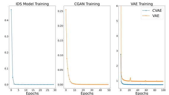
Fig. 3. Loss function with the training epochs for the (a) Feedforward IDS network (b) cGAN discriminator training (c) VAE and CVAE training.
