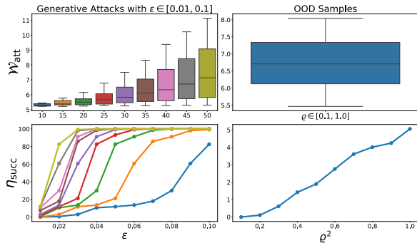
Fig. 4. (a) Distributional distance between X_{\text{adv}} and X_{\text{att}} with various refinements. (b) Distributional distance between X_{\text{ood}} and X_{\text{att}} with various refinements. (c) Attack success rate for different refinements (c) Attack success rates for different OOD samples.
