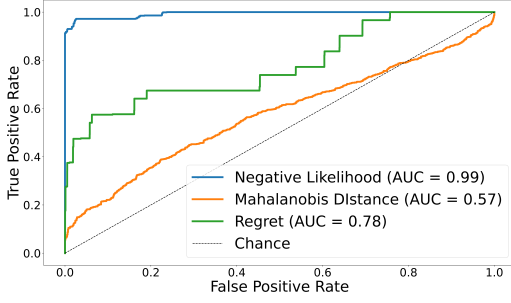
Fig. 7. ROC curve for detecting adversarial samples from OOD samples.
