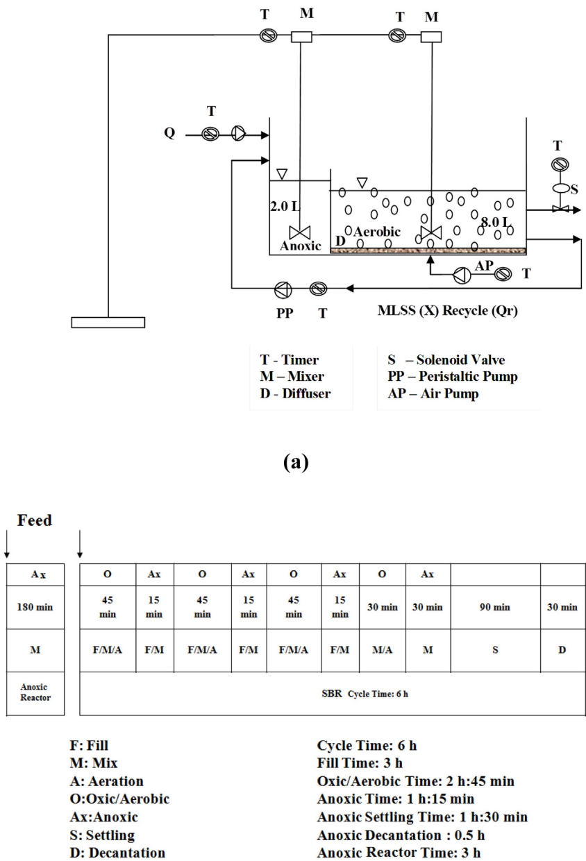
Fig. 1. (a) Schematic diagram of reactor set up (b) Reaction cycle in sequencing batch reactor with Pre-anoxic tank.
