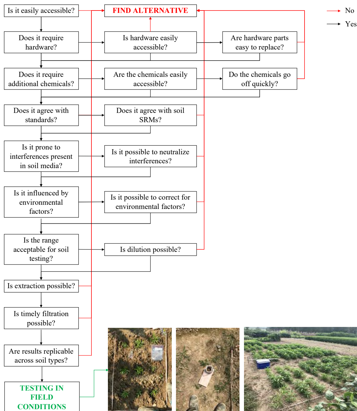
Fig. 6. Proposed testing sequence of laboratory experiments to be undertaken as part of field test kit development. Terms used: SRM – soil reference material; additional chemicals encompass chemicals required for the test strip reaction to occur, and chemicals used during the extraction process; environmental factors refer primarily to temperature and humidity.
