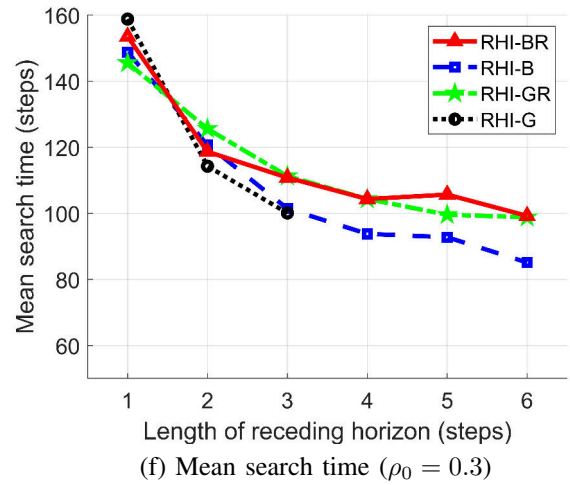
Fig. 9. The results of Monte Carlo simulation with various approximation methods and horizon length under obstacle maps.
