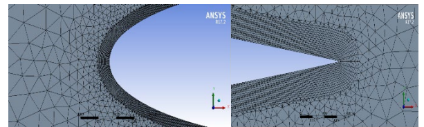
Fig. 4. Zoom-in Boundary Layer. Left: Leading Edge Foil; Right: Trailing Edge Foil.
