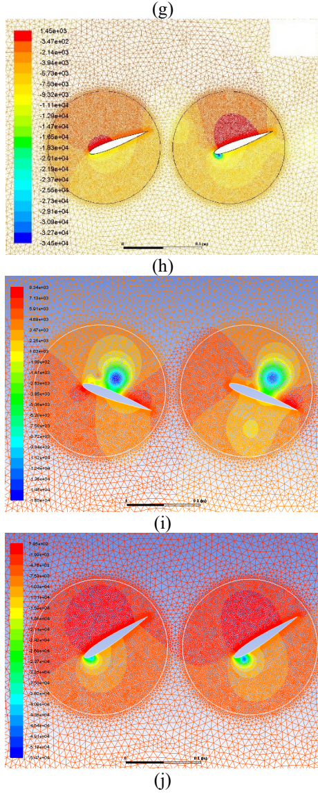
Fig. 9. (a) C_{lFA} maximum when f^* = 0.04 ; (b) C_{lFA} minimum when f^* = 0.04 ; (c) C_{lRA} maximum when f^* = 0.04 ; (d) C_{lRA} minimum when f^* = 0.04 ; (e) C_{lFA} maximum when f^* = 0.14 ; (f) C_{lFA} minimum when f^* = 0.14 ; (g) C_{lRA} maximum when f^* = 0.14 ; (h) C_{lRA} minimum when f^* = 0.14 ; (i) C_{lFA} and C_{lRA} maximum when f^* = 0.18 ; (j) C_{lFA} and C_{lRA} minimum when f^* = 0.18 .
