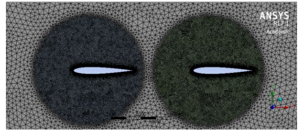
Fig. 3. Meshing of 2D Tandem NACA0012 Foils.
