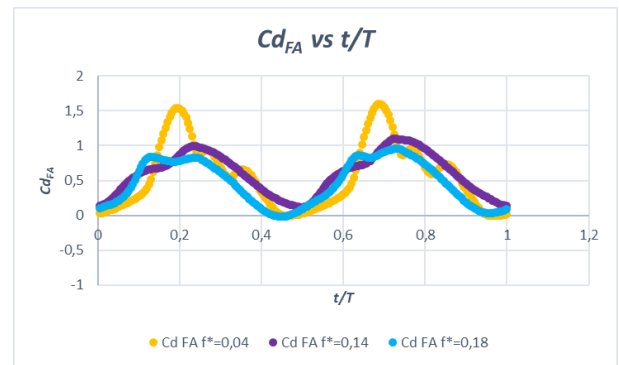
Fig. 7. C_{d,FA} vs t/T on parametric study f^* .
