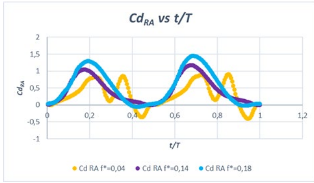
Fig. 8. C_{dRA} vs t/T on parametric study f^* .
