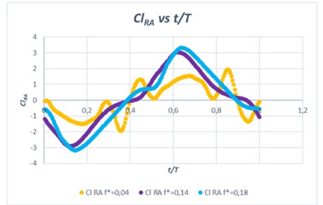
Fig. 11. C_{lRA} vs t/T on parametric study f^* .
