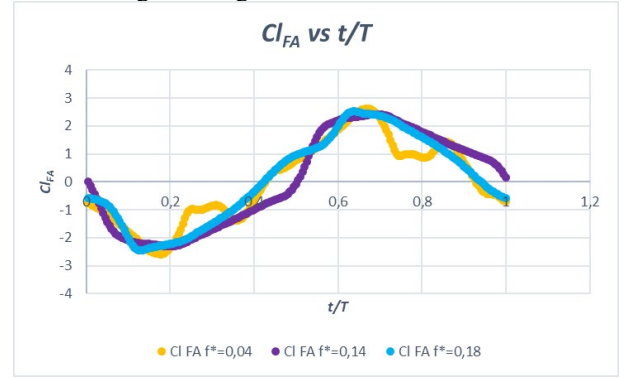
Fig. 10. C_{lFA} vs t/T on parametric study f^* .
