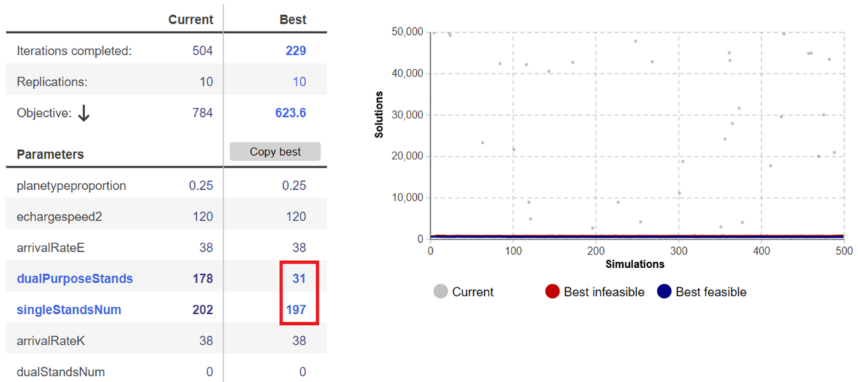
Fig. 7. shows the AnyLogic GUI containing the scatter search plot of simulation solutions (right). Here, the x-axis represents simulation runs, and the y-axis represents current solution, best feasible solution (blue plot) and best infeasible solution (red plot) found for each simulation based on their objValue values. The optimal best-case single / dual purpose stand numbers (boxed in red) generated during the optimisation experiment run for London Heathrow based on a charging regime of 120 minutes for a 25% increase in electric aircraft operations is shown to the left.
