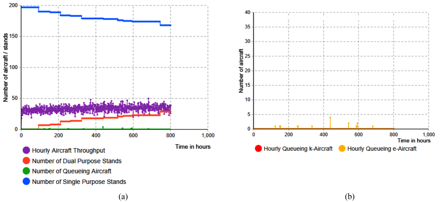
Fig. 6. shows the following plots for a 25% increase in the proportion of electric aircraft movements: (a) plot showing: the hourly throughput of all aircraft, number of queueing aircraft recorded per hour, number of dual-purpose stands, number of single purpose stands (y-axis – number of aircraft/stands, x-axis – time in hours); (b) plot showing: hourly queueing for kerosene vs electric aircraft (y-axis – number of aircraft/arrival rates, x-axis – time in hours).
