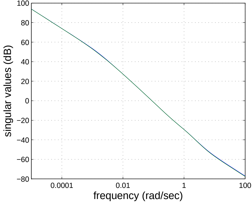
Figure 10: Open-loop singular values.
