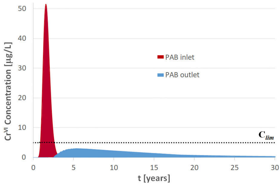
Figure 9. PAB maximum inlet and outlet \text{Cr}^{\text{VI}} concentrations over the time, respectively at points A and B.
