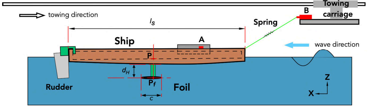
FIG. 3. Schematic sketch about experimental setup.
