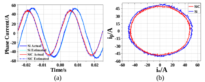
Fig. 21. Phase current and \alpha\beta current waveforms under 800rpm and 24N·m of the motor. (a) Phase current waveforms. (b) \alpha\beta current waveforms.
