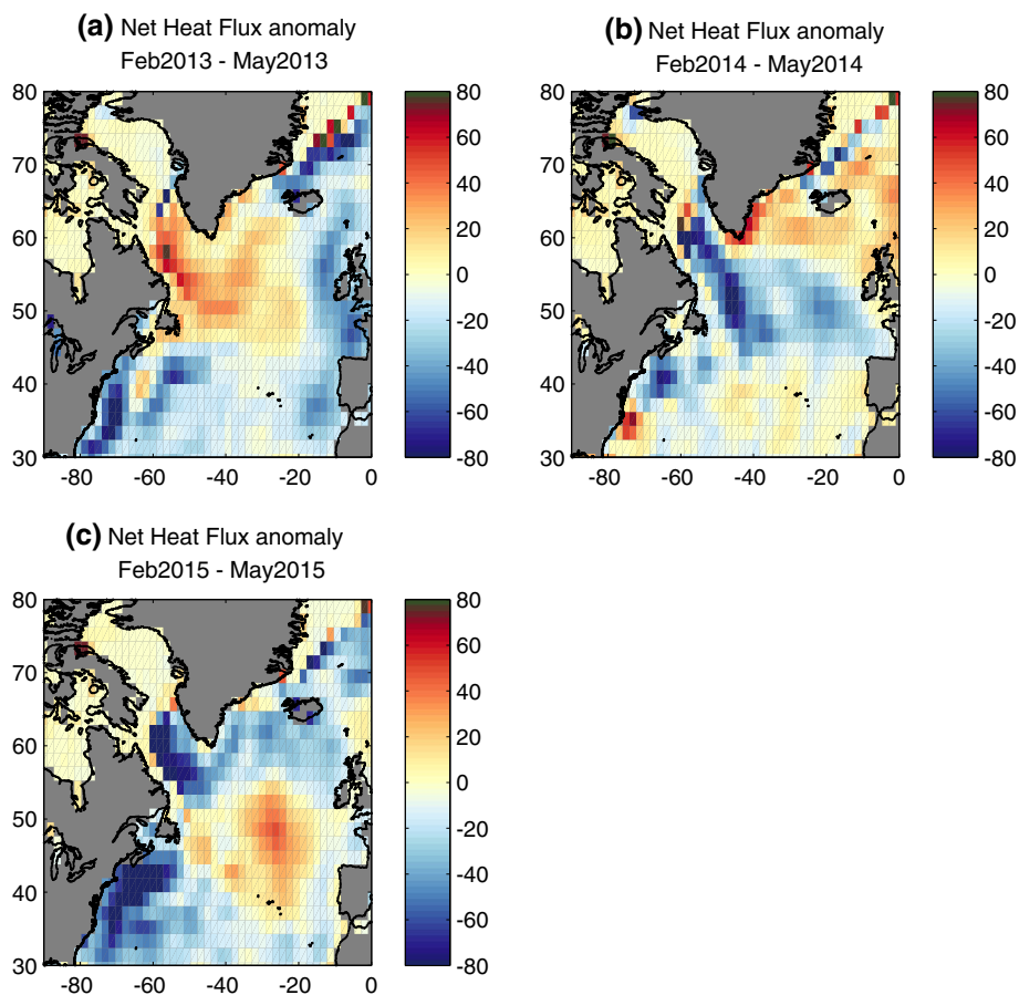
Fig. 14 Anomalies (relative to 1981–2010) of net air–sea heat flux ( \text{W m}^{-2} ), averaged over February–May of: a 2013; b 2014; c 2015
