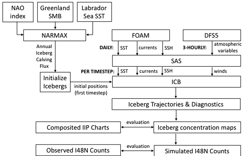
Fig. 1 Model components, forcing, outputs and evaluation
