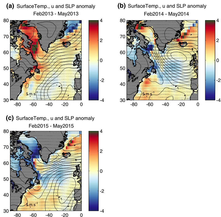
Fig. 4 Oceanographic and meteorological conditions in the North Atlantic, averaged for February–May of: a 2013, b 2014, c 2015. Shading shows SST anomaly (°C), contours show sea level pressure anomaly (mb), and arrows show wind speed anomaly, all defined relative to 1981–2010
