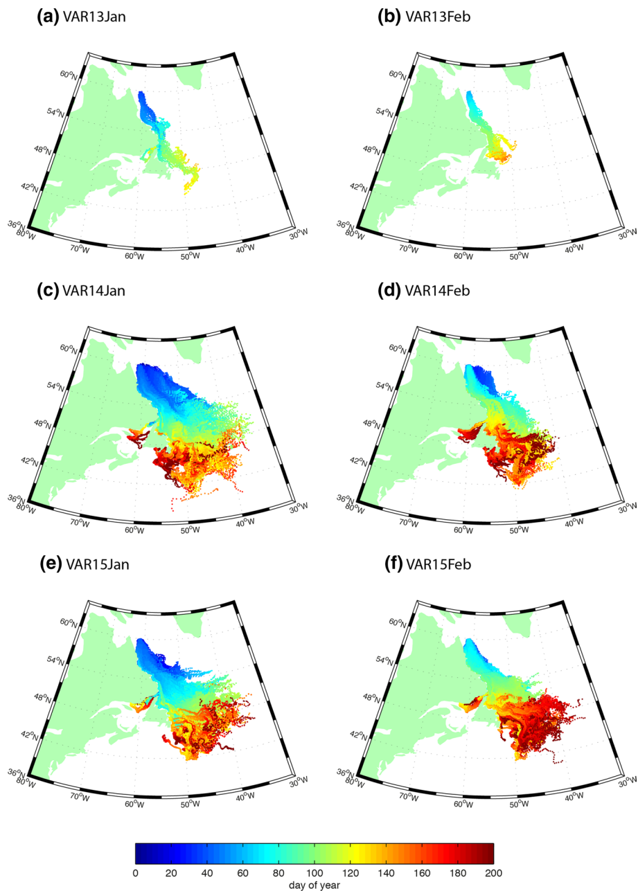
Fig. 5 Simulated iceberg trajectories, daily positions 2013–2015, colour-coded for day of year: a, c, e January starts; b, d, f February starts
