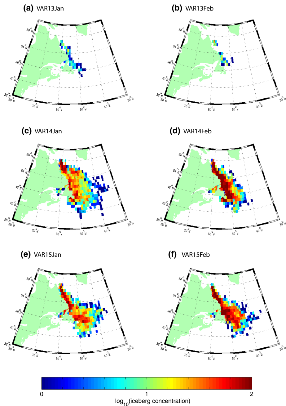
Fig. 6 Simulated iceberg distributions, 2013–2015, colour-coded for cumulative number per 1^\circ grid square (sampling as for IIP data—see Fig. 1): a, c, e January starts; b, d, f February starts
