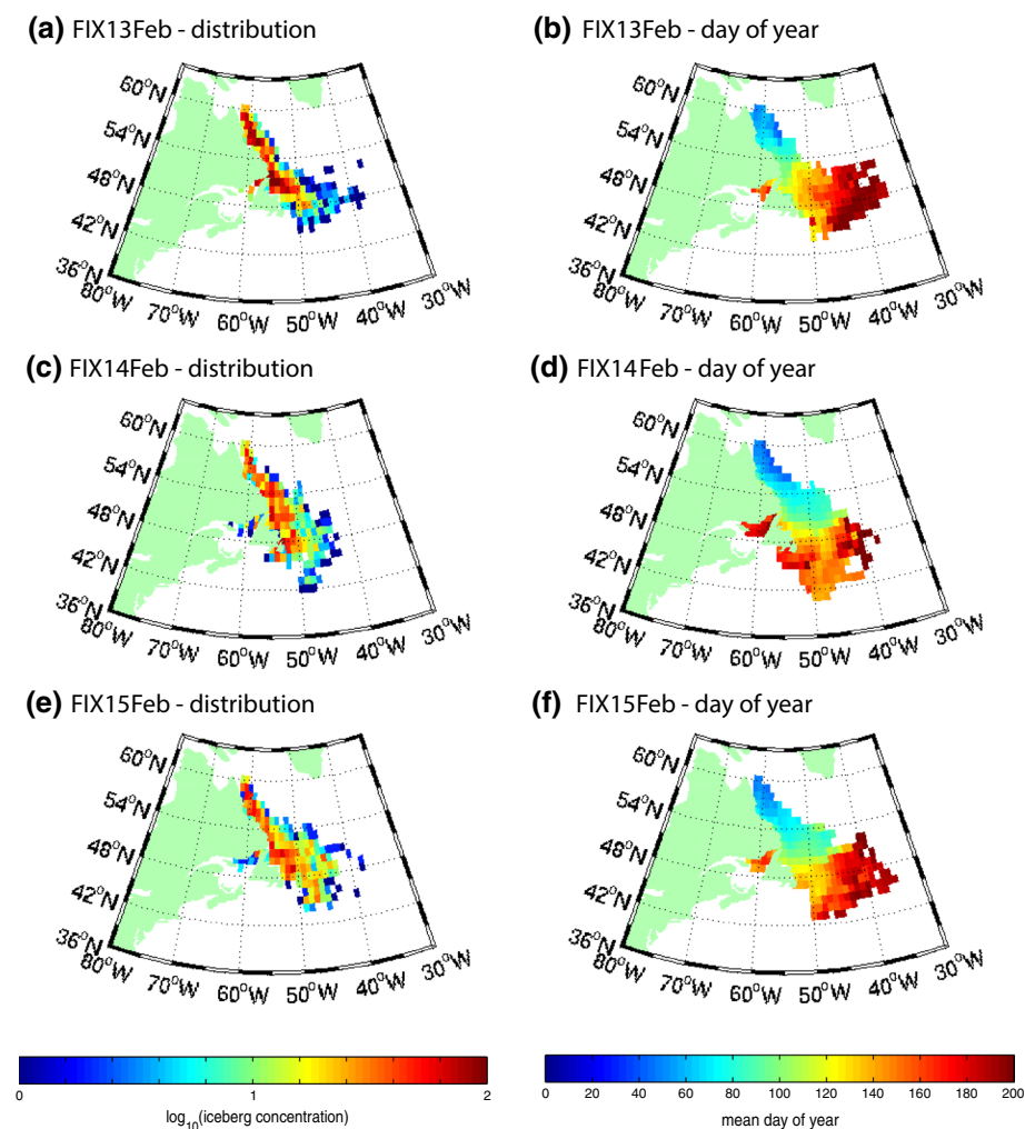
Fig. 12 Simulated iceberg distributions, climatological February iceberg fluxes: a, c, e colour-coded for cumulative number per 1° grid square; b, d, f colour-coded for day of year
