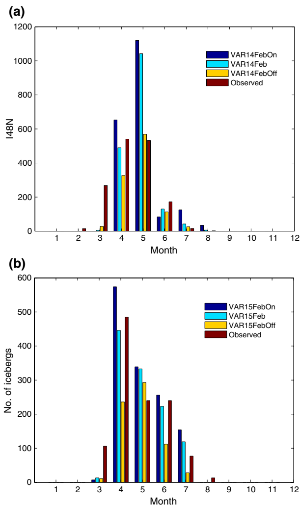
Fig. 11 As Fig. 10, for prescribed February iceberg fluxes at 60°N, at the default longitude, shifted 1° on/offshore, and observed: a 2014; b 2015
