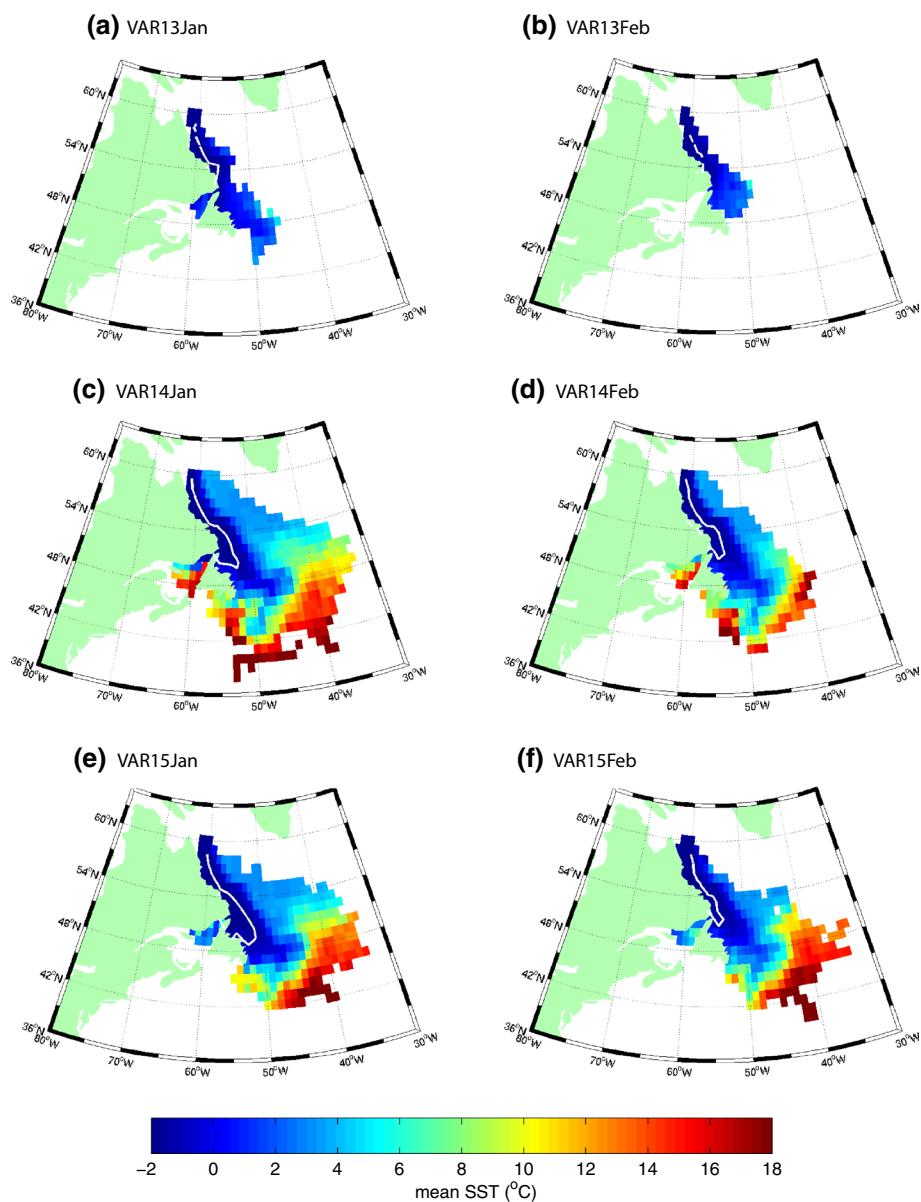
Fig. 9 As Fig. 6, colour-coded for sea surface temperature, indicating the -1.5^{\circ}\text{C} isotherm with the thick white line
