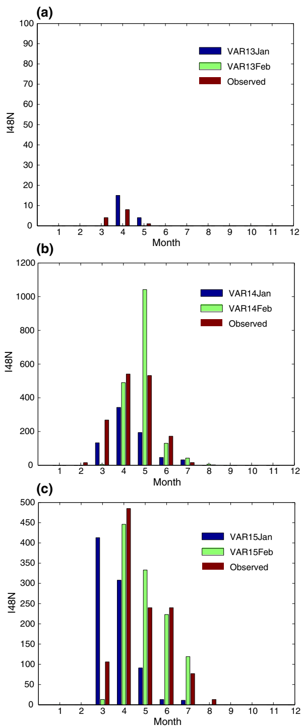
Fig. 10 Number of icebergs crossing 48°N, monthly over 2013–2015, in simulations with variable iceberg fluxes at 60°N (blue bars—January fluxes; green bars—February fluxes), and observed (red bars): a 2013; b 2014; c 2015
