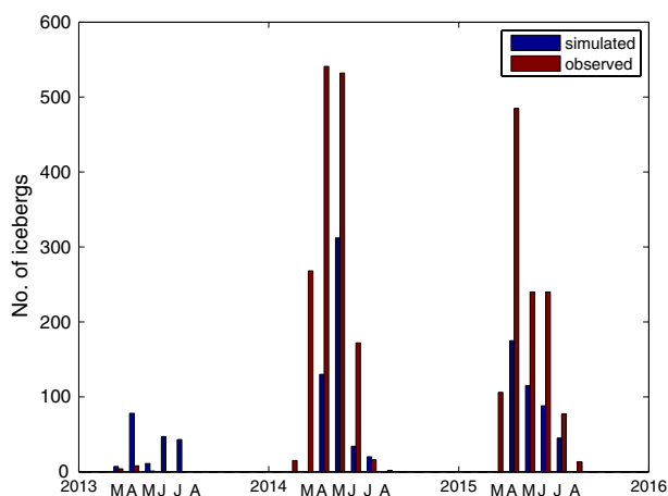
Fig. 13 Number of icebergs crossing 48°N, per month over 2013–2015, in simulations with climatological February iceberg fluxes at 60°N (blue bars), and observed (red bars)
