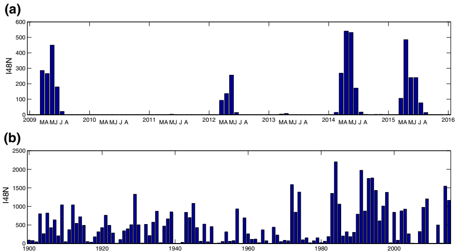
Fig. 3 Number of icebergs observed crossing 48°N: a monthly over 2009–2015 (labelling March–August) and b annually over 1900–2015
