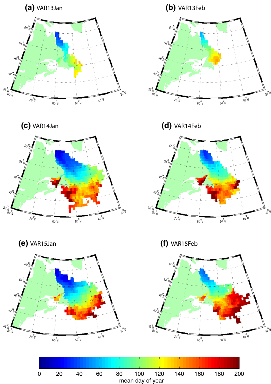
Fig. 7 As Fig. 6, colour-coded for day of year
