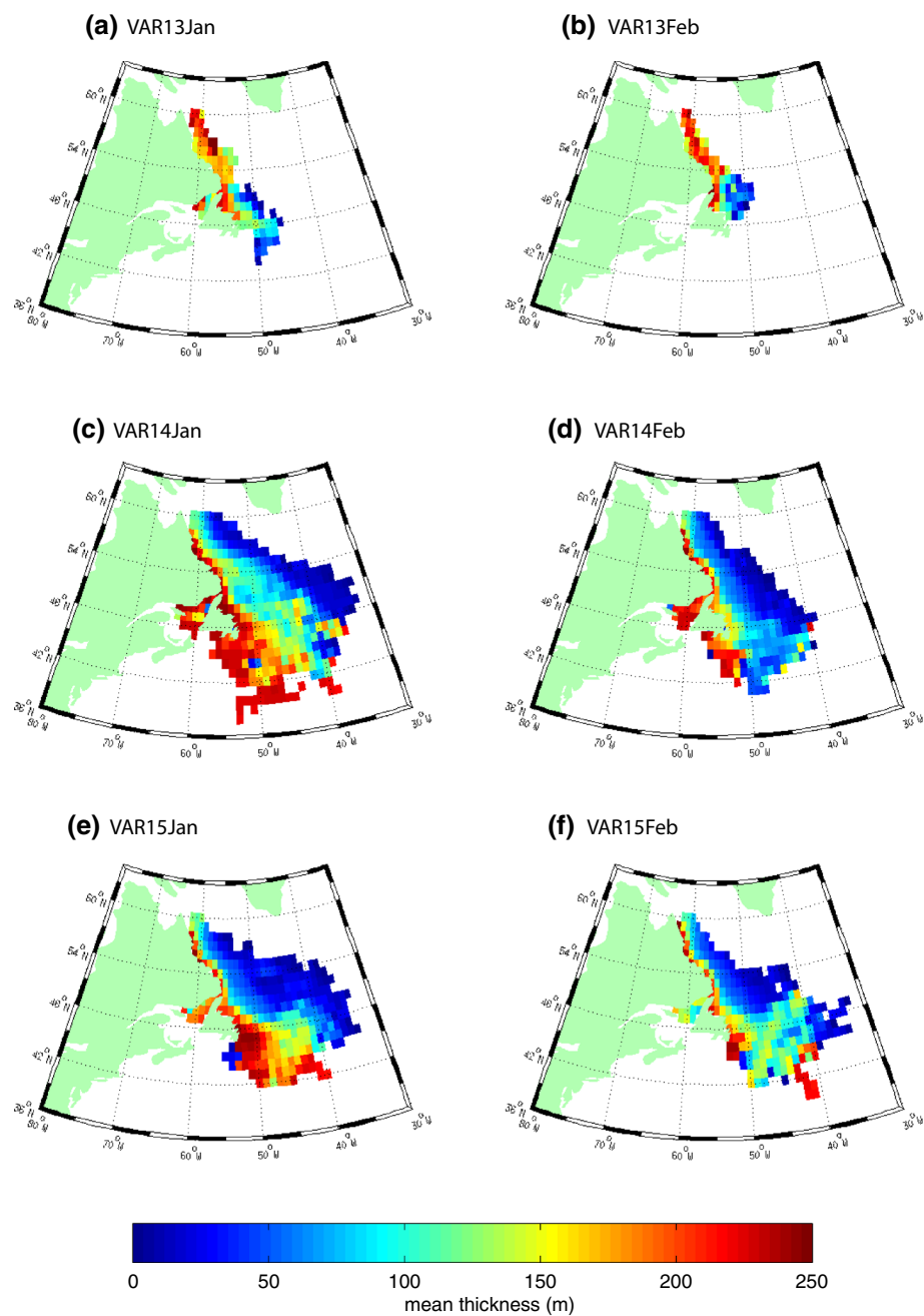
Fig. 8 As Fig. 6, colour-coded for thickness
