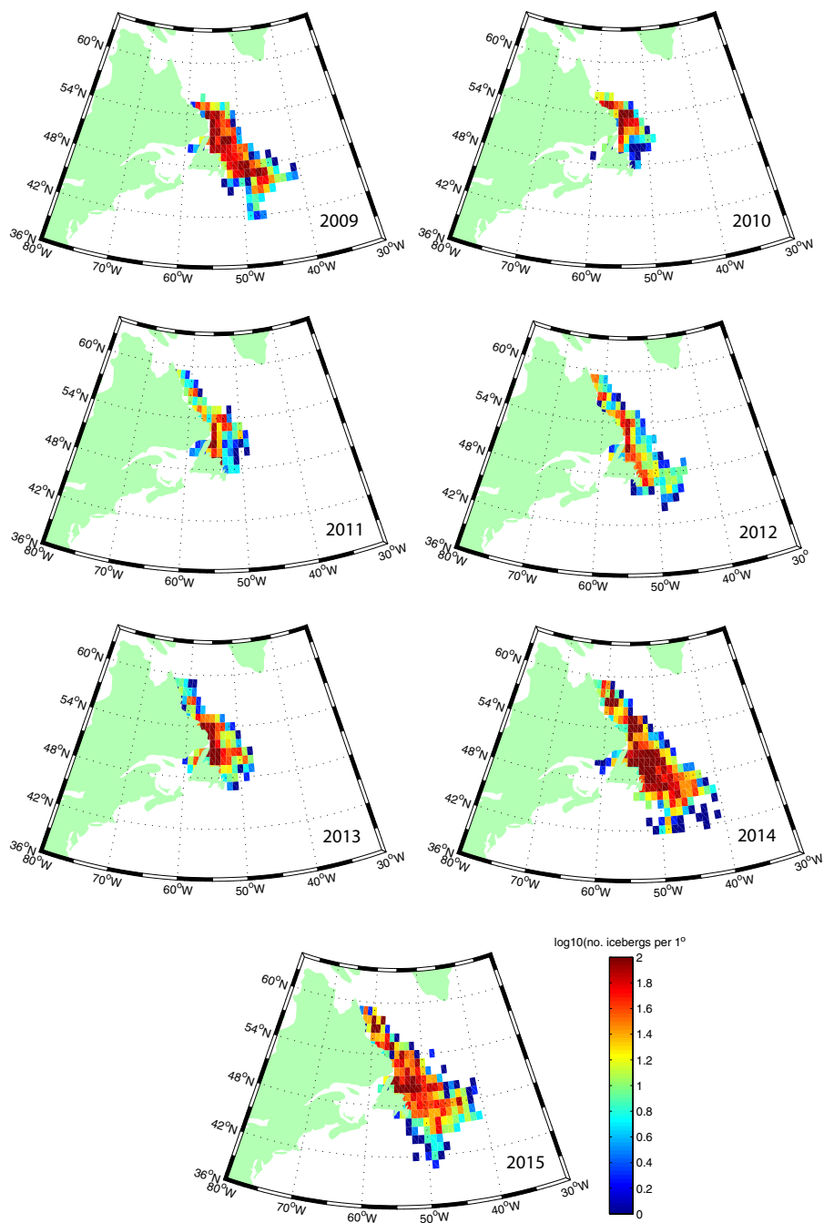
Fig. 2 Digitized IIP iceberg distributions 2009–2015, colour-coded for cumulative number per 1° grid square, sampling the 15th day of each month
