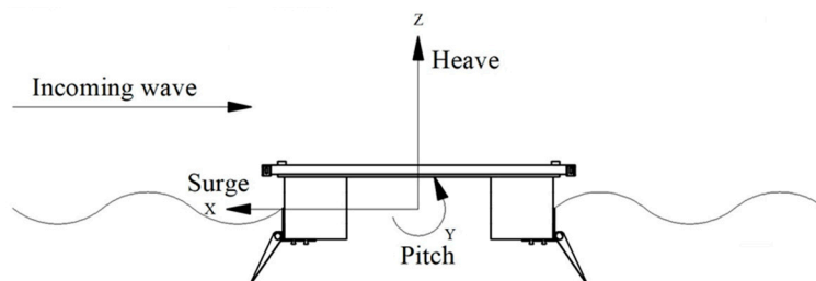
Figure 7. Motion schematics of the floating breakwater.
