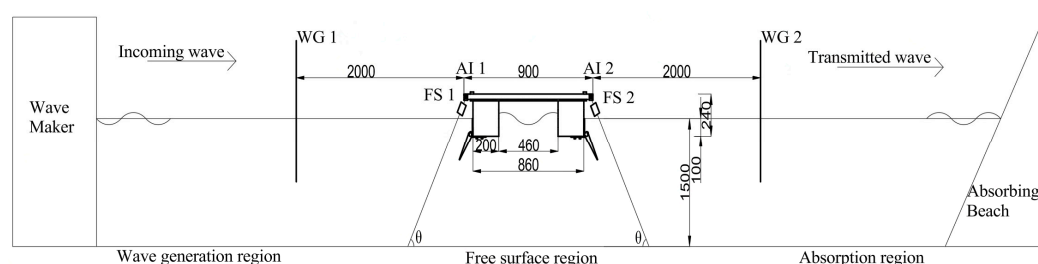
Figure 6. Illustration of the experimental setup.
