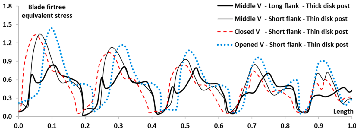
Fig. 7. Stress distribution of serrations.
