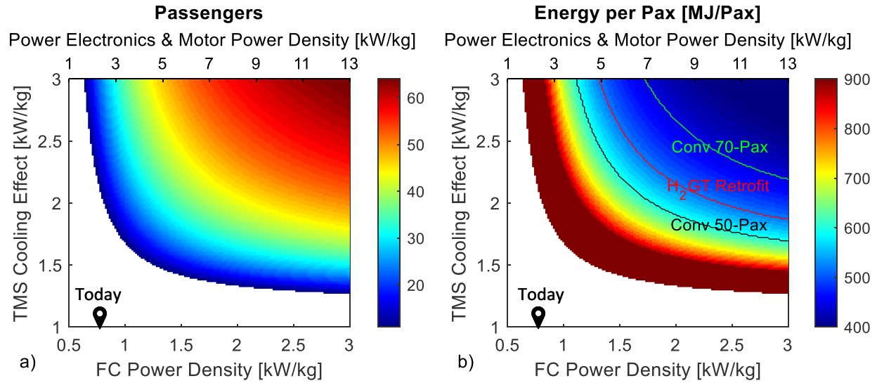
Fig. 18 Number of passengers and energy per passenger for 300nmi and MTOW over a range of TMS, FC, motor and power electronics power density
