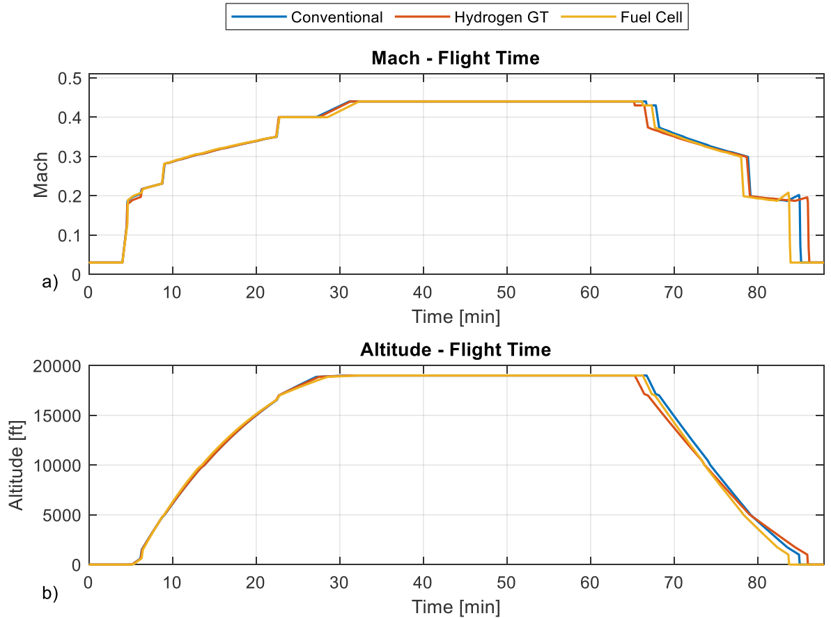
Fig. 10 Flight mission profile (Mach and Altitude)
