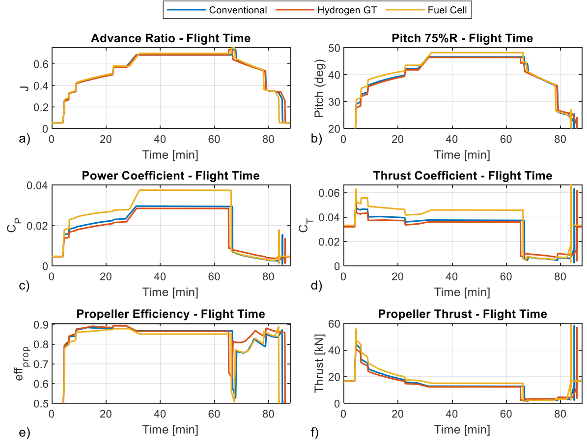
Fig. 12 Variable pitch propeller performance over flight time
