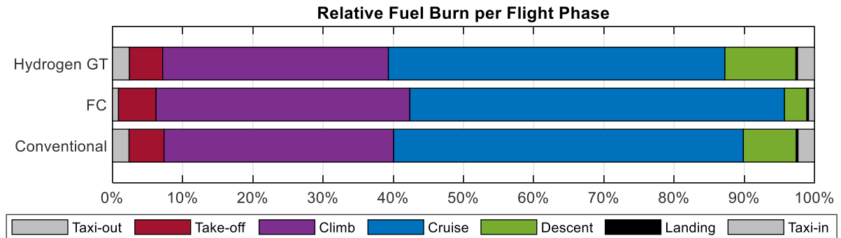
Fig. 16 Relative fuel/energy consumption per flight phase
