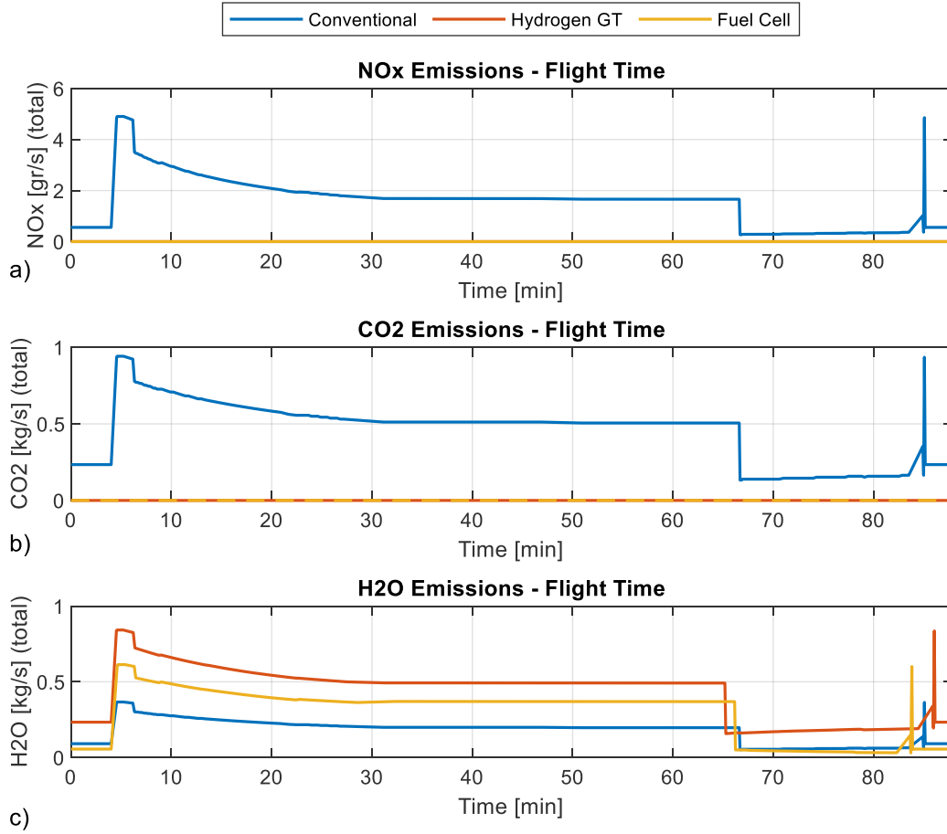
Fig. 15 Emissions produced by the conventional regional aircraft, the hydrogen GT aircraft and the FC fully-electric aircraft
