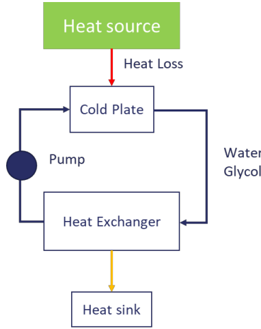
Fig. 7 Liquid cooling system for thermal management system
