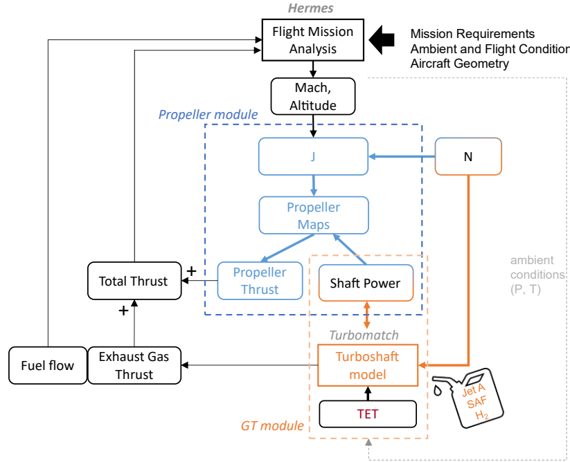
Fig. 8 Integration flowchart for GT-Variable Pitch Propeller-Aircraft system within the flight mission analysis platform
