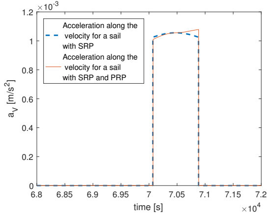
Figure 10: Tangential acceleration around the periapsis for a sail with SRP and SRP+PRP for a sail around the Earth on T2 ( \omega_0 = 90 deg) considering SRP+PRP.
