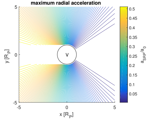
(b) Contour of a_{SRP}/a_0 .
