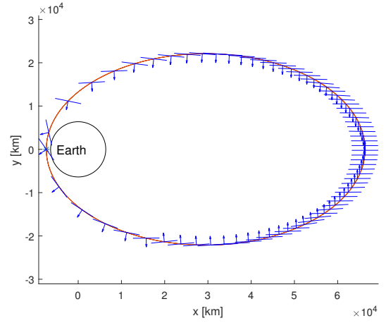
Figure 11: Trajectory around the Earth with orientation of the sail on T3 ( \omega_0 = 180 deg) considering SRP+PRP.
