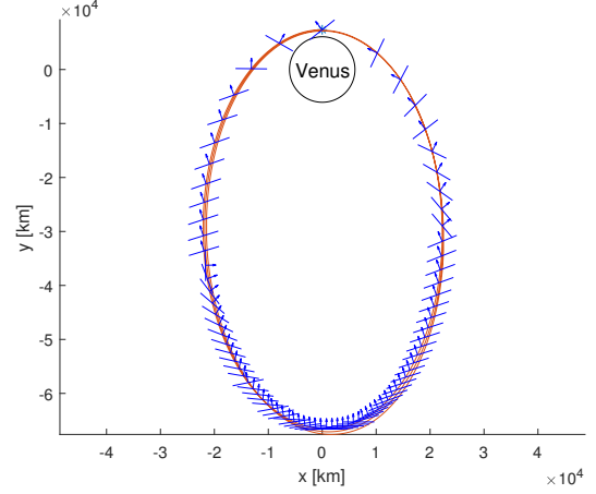
Figure 14: Trajectory around Venus with orientation of the sail on T2 ( \omega_0 = 90 deg) considering SRP+PRP.
