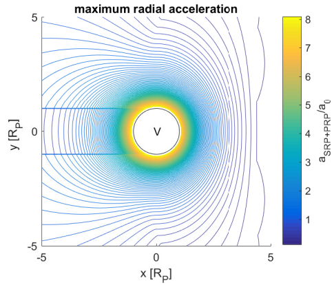
(b) Contour of a_{SRP+PRP}/a_0 .
