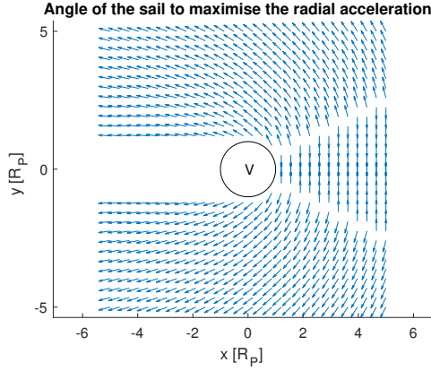
(a) Direction of the sail normal.
