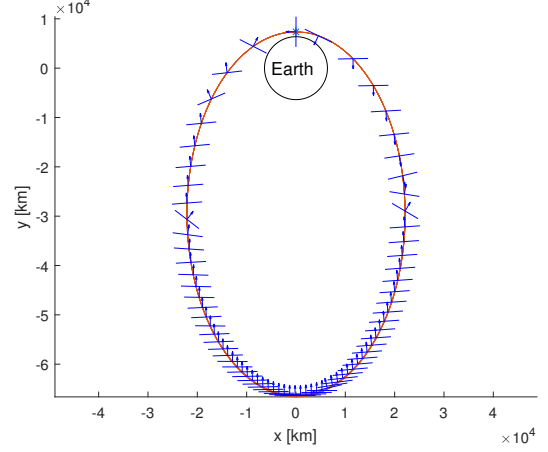
Figure 8: Trajectory around the Earth with orientation of the sail on T2 ( \omega_0 = 90 deg) considering SRP+PRP.
