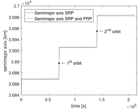
Figure 9: Semi-major axis with SRP and SRP+PRP for a sail around the Earth on T2 ( \omega = 90 deg).
