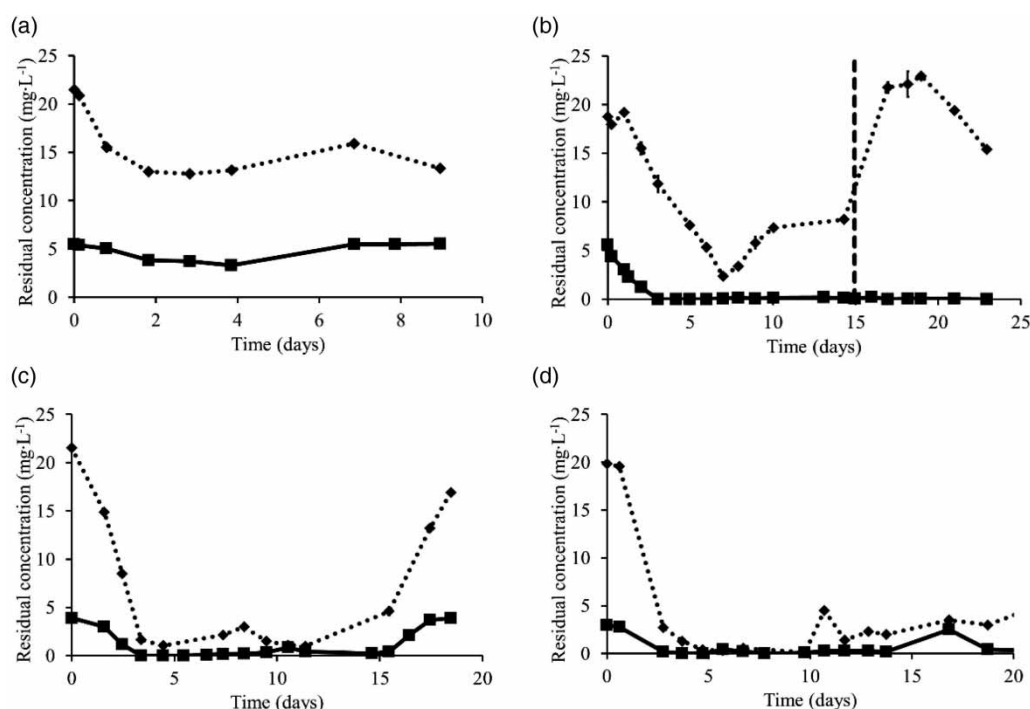
Figure 3 | Ammonium and nitrate remediation for site A samples for (a) 3 h, (b) 6 h (addition of fresh feed on day 15.0), (c) 12 h and (d) 20 h HRT. \text{NH}_4\text{-N} (■) and \text{NO}_3\text{-N} (◆). Average influent concentration 4.2 \text{ mg}\cdot\text{L}^{-1} \text{ NH}_4\text{-N} and 20.3 \text{ mg}\cdot\text{L}^{-1} \text{ NO}_3\text{-N} .
