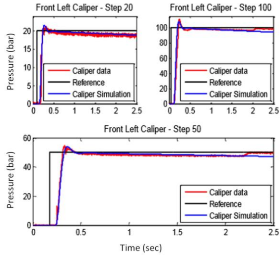
Fig 7. Brake Caliper Experimental and Simulation data (Martínez, et al., 2014)
