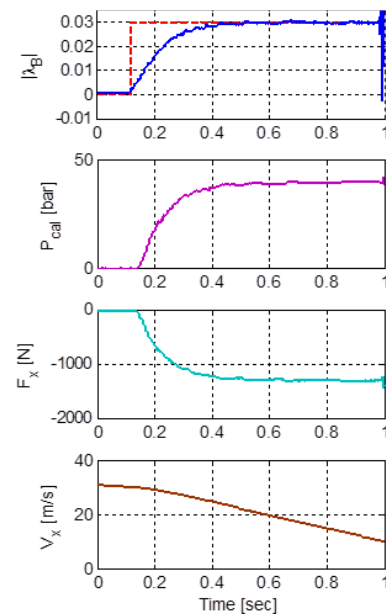
Figure 8: HiL test results for the closed loop slip control system (Soltani & Assadian, 2015)
