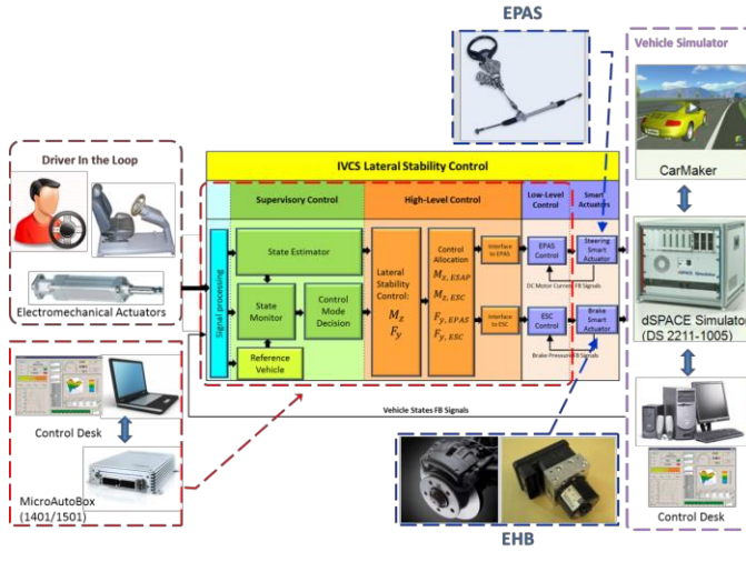
Fig. 4. The integrated steering & brake HiL architecture
