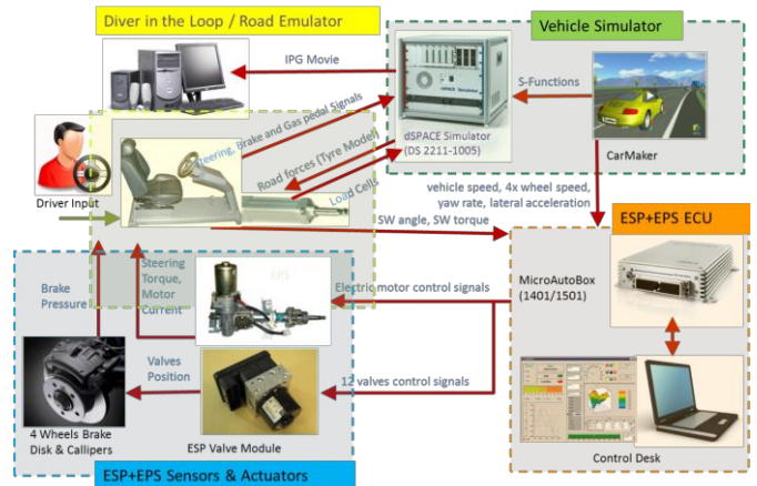
Fig. 5. The signal flows among several HiL components
