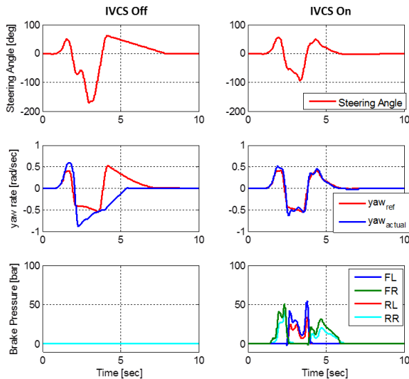
Fig 9. HiL test results of the Integrated Vehicle Dynamics Control System (IVCS) subject to VDA lane-change manoeuvre (Soltani, 2014)
