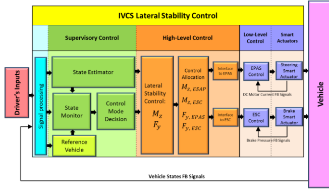
Fig. 3. Customised IVCS control structure
