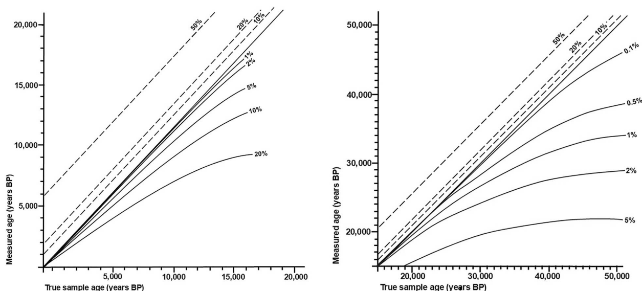
Figure 1. Theoretical relationships between true and measured radiocarbon ages for samples contaminated with ‘modern’ and ‘dead’ carbon, for the a. 0–16,000 year range and b. the 12–50,000 year range. Redrawn from Gillespie (1984). The thick solid line shows the relationship between true sample age and measured sample age for uncontaminated samples. The thin solid lines show the effect of contamination by ‘modern’ carbon (130% of the modern reference standard, about the atmospheric level in 1984). The dotted lines show the effect of contamination by ‘dead’ carbon (containing no ^{14}\text{C} ).
