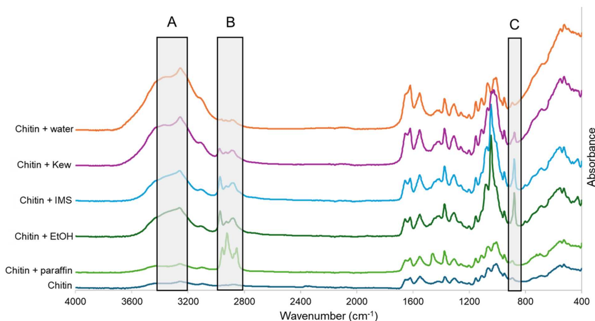
Figure 3. FTIR spectra (staggered for ease of viewing) of paraffin and other storage media on commercially-available chitin from shrimp. Region A (3400–3200 \text{cm}^{-1} ) is dominated by a broad OH peak; Region B highlights key peaks associated with organic storage media or paraffin between 2950–2850 \text{cm}^{-1} ; Region C highlights key peak at c. 880 \text{cm}^{-1} .
