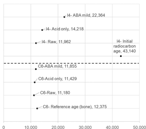
Figure 2. Measured radiocarbon ages for samples paraffin floated and then stored in industrial methylated spirits since 1956 (Isleworth, Coope and Angus 1975) and 1986 (Condoover, Scourse et al. 2009). C6 is Condoover 6; I4 is Isleworth 4. Note that the actual age of sample I4 is likely beyond the radiocarbon limit at c. 70–100,000 years BP. Sample details in text.
