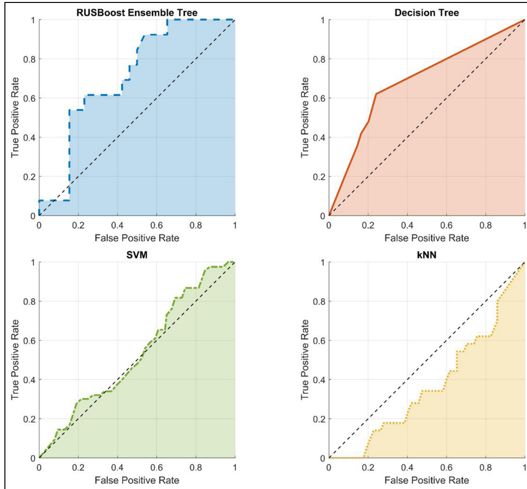
Figure 8. ROC curves with shaded AUC regions for the four classifiers under 10-fold cross validation.
