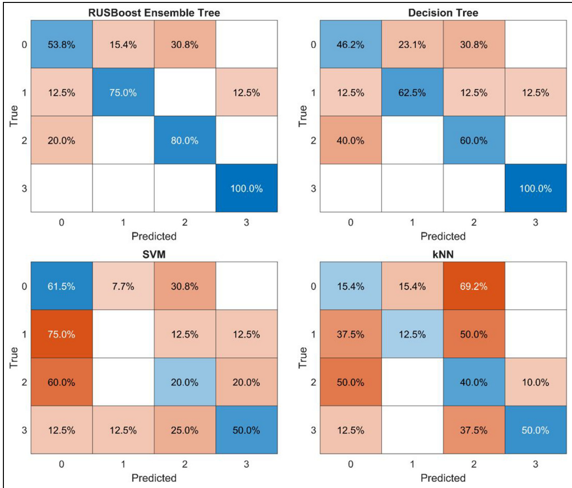
Figure 7. Confusion matrices for the four classifiers under 10-fold cross validation.
