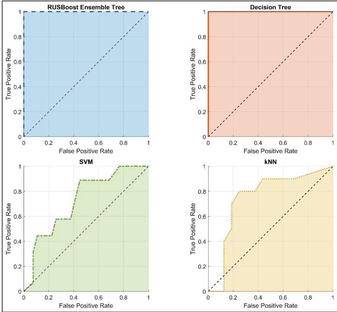
Figure 4. ROC curves with shaded AUC regions for the four classifiers under single-run (hold-out) evaluation.
