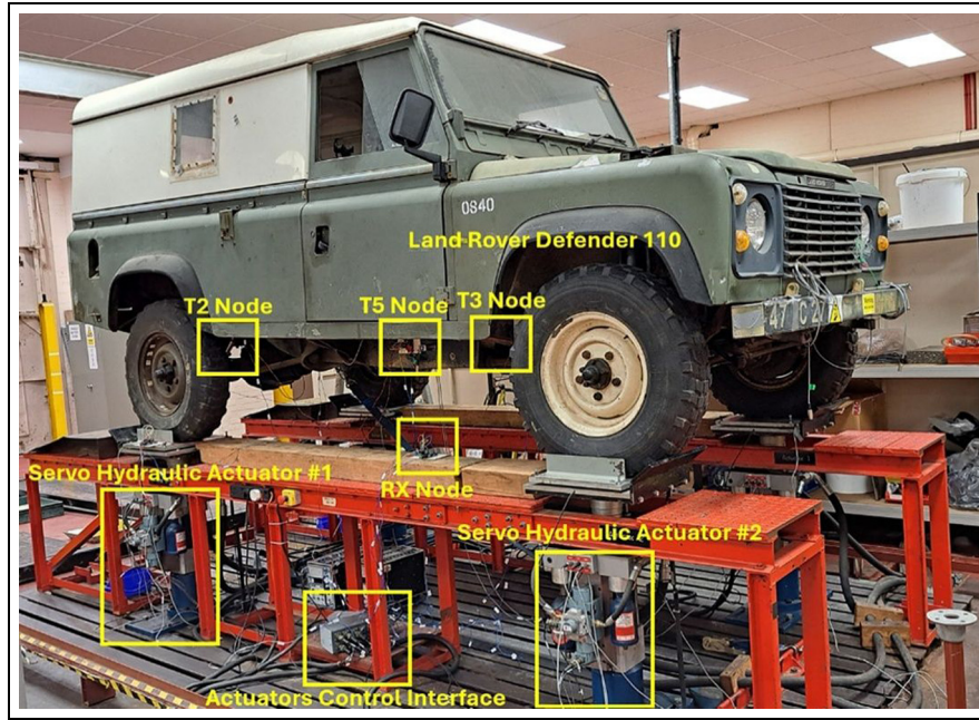
Figure 1. Experimental setup showing the distributed sensor architecture installed on the Land Rover Defender 110.
