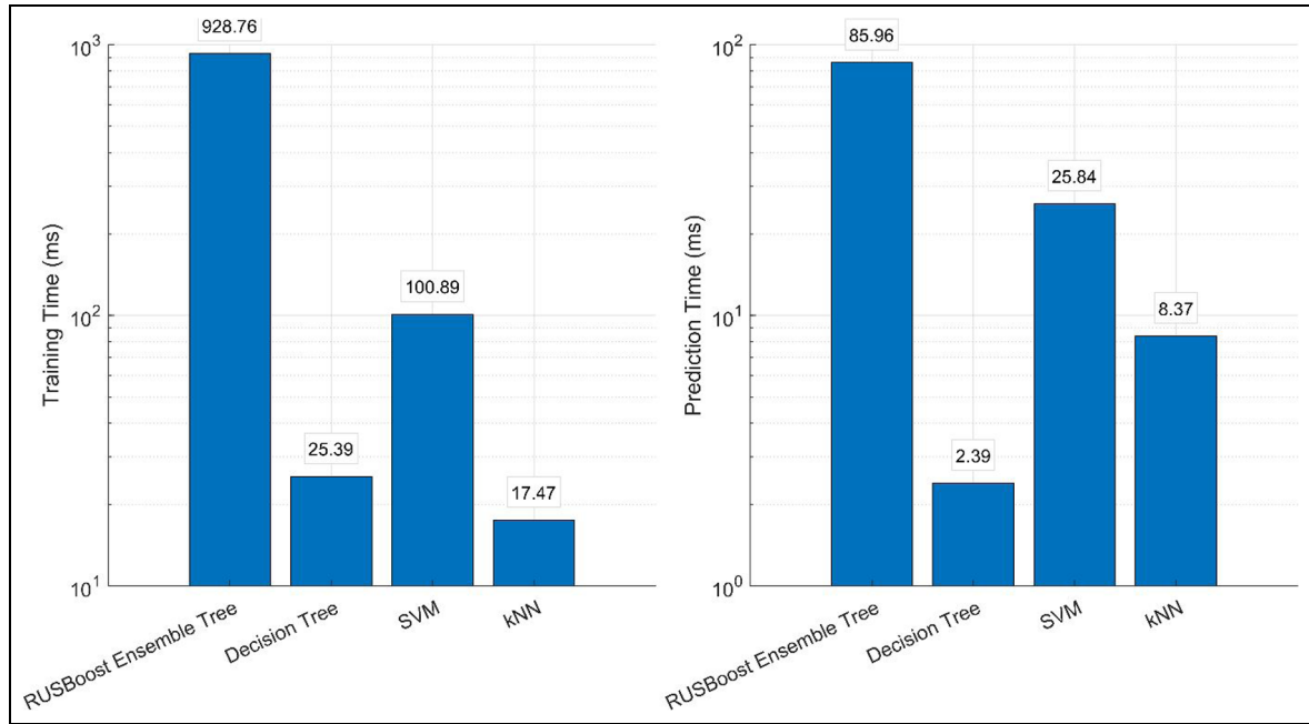
Figure 9. Comparison of training and prediction times for the evaluated classifiers.
