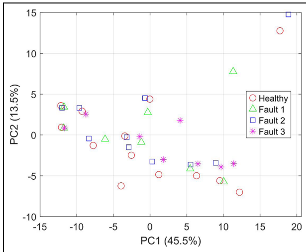
Figure 6. PCA projection of the feature space for single run evaluation, showing class distribution and overlap.
