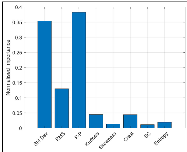
Figure 5. Normalised out-of-bag (OOB) permutation feature importance derived from the ensemble classifier.
