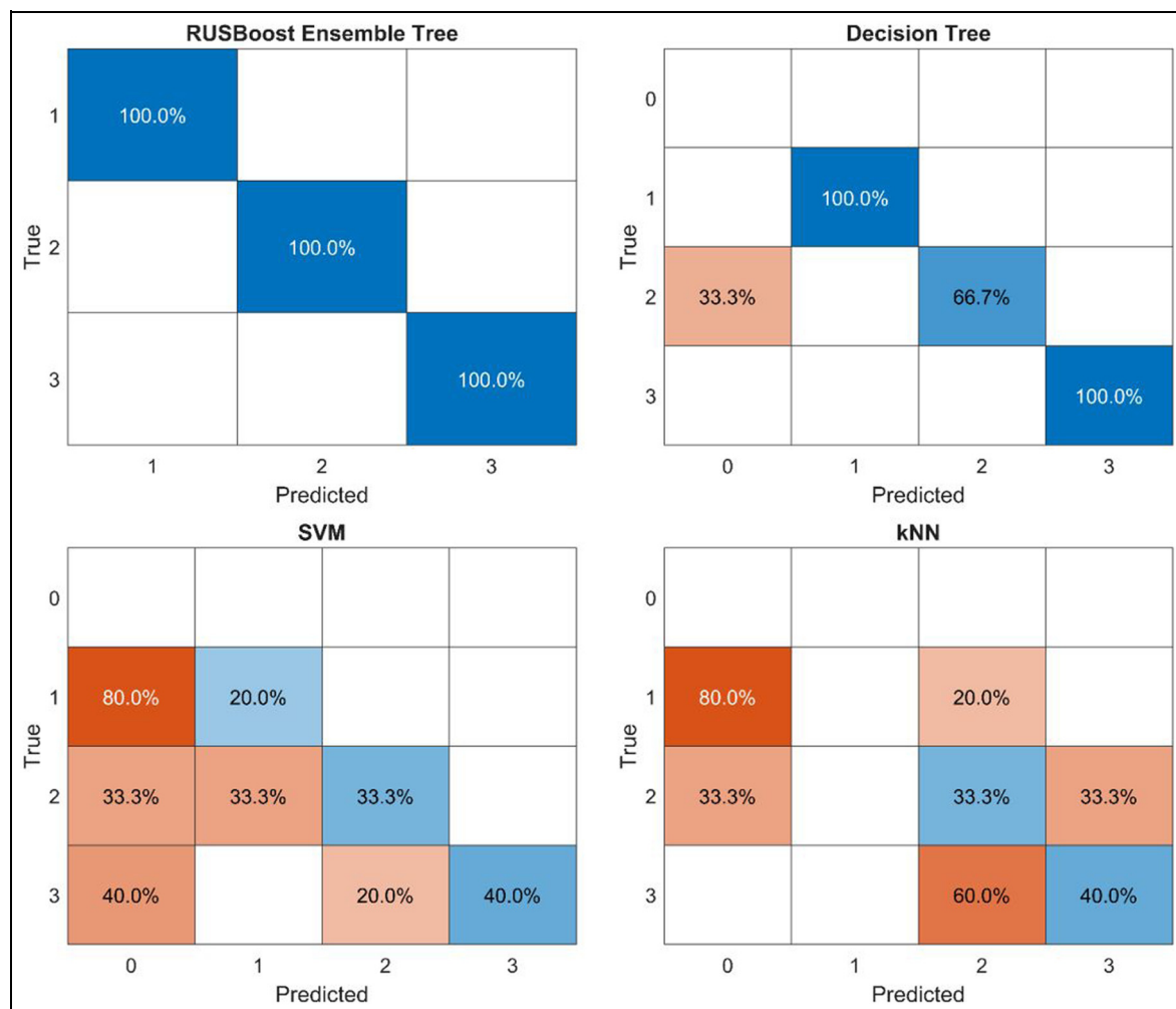
Figure 3. Normalised confusion matrices for the four classifiers under single-run (hold-out) evaluation.
