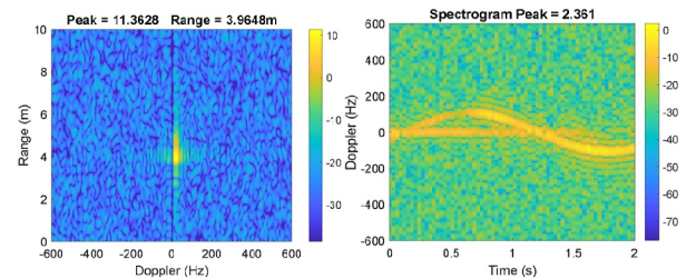
FIGURE 14 | VV-polarisation of a nano-drone response.
