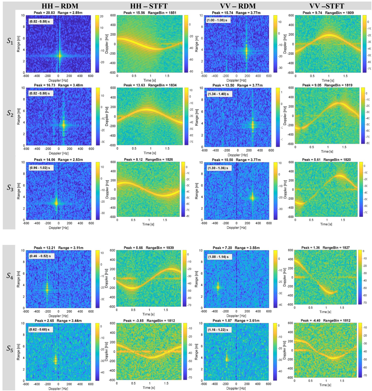
FIGURE 5 | Front-to-back oscillation with a window length of 30 ms for the STFT analysis.
