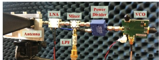
FIGURE 2 | A close-up of a K-band radar system developed.
