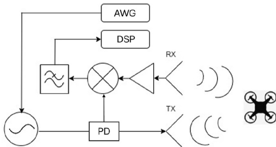
FIGURE 1 | Block diagram of K-band radar prototype.
