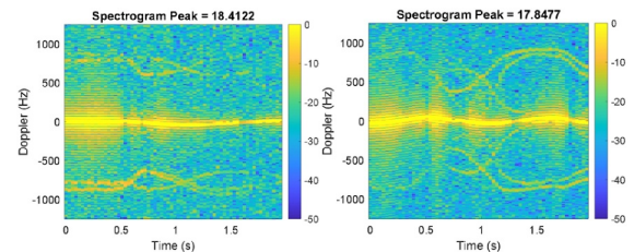
FIGURE 15 | Observed Jet engine modulation (JEM) features in the nano-drone Doppler return.
