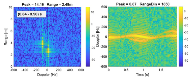
FIGURE 11 | Side-to-side oscillation of multiple targets in a VV-polarisation.
