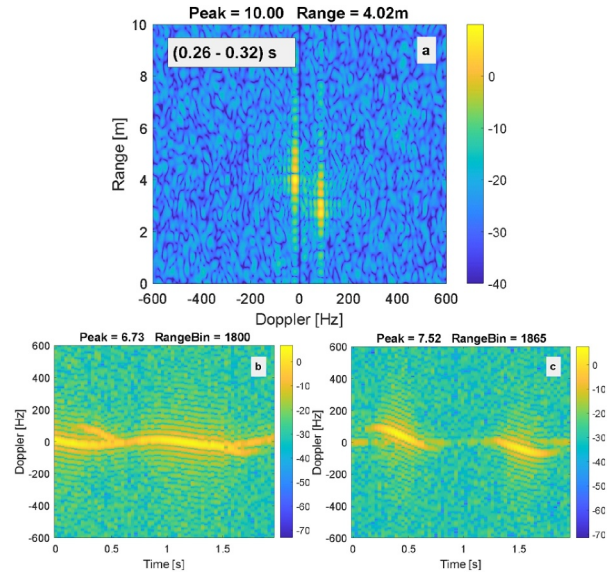
FIGURE 10 | Side-to-side oscillation of multiple targets in an HH-polarisation.
