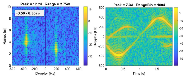
FIGURE 9 | Front-to-back oscillation of multiple targets in a VV-polarisation.
