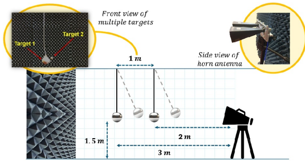
FIGURE 7 | Experimental arrangement of multiple bearing spheres. Target 1 is S_2 and Target 2 is S_3 .
