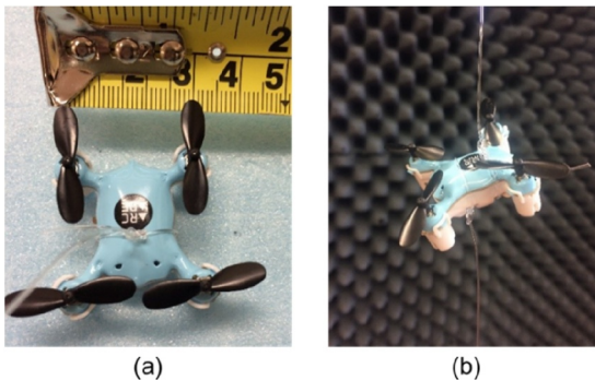
FIGURE 12 | (a) Close-up of ARCADE nano-drone and (b) the target hanging for data collection.
