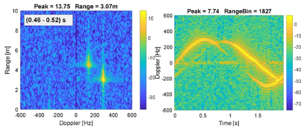
FIGURE 8 | Front-to-back oscillation of multiple targets in an HH-polarisation.
