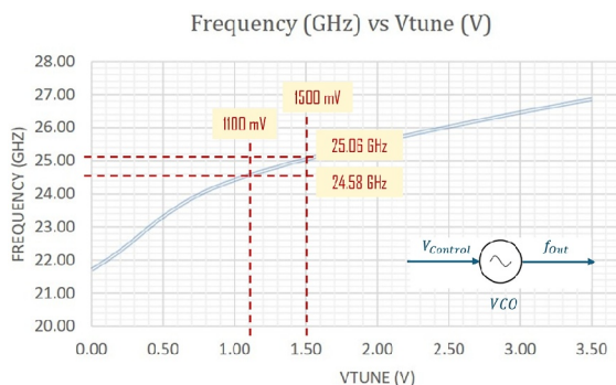
FIGURE 3 | Characteristic curve of the VCO.
