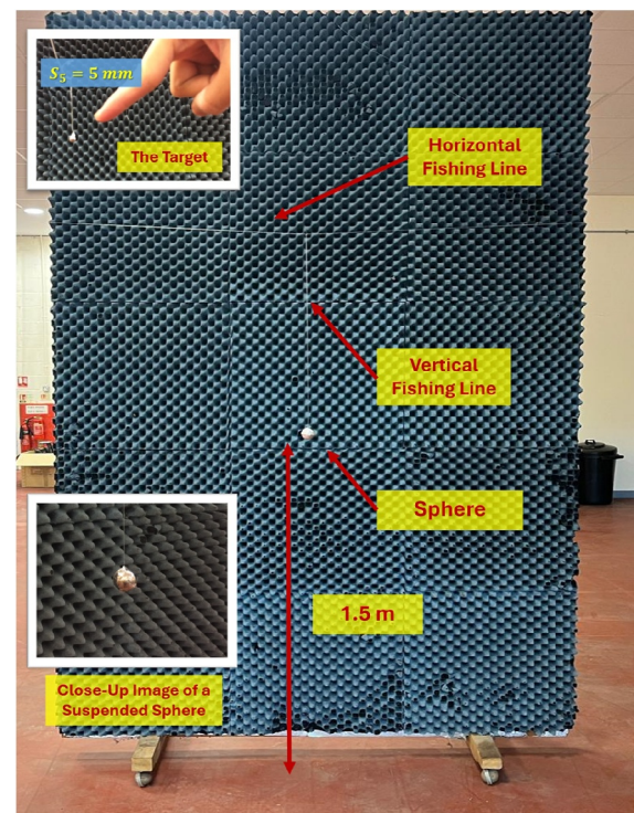
FIGURE 4 | Experimental arrangement showing the positioning of a single suspended sphere.
