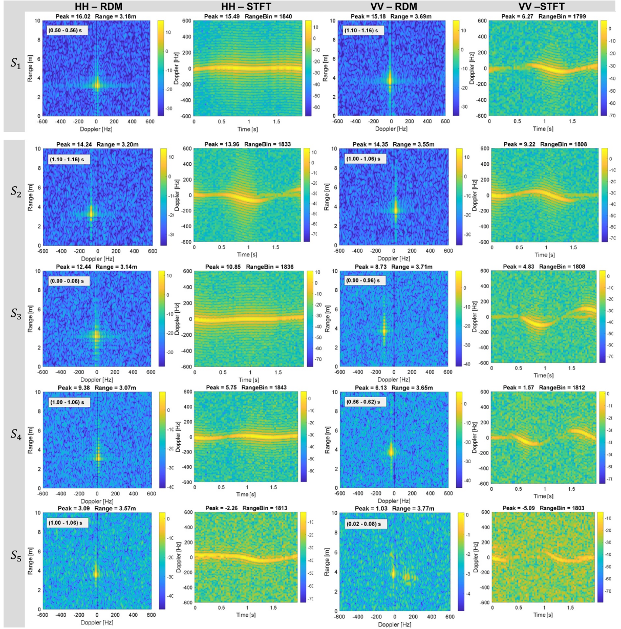
FIGURE 6 | Side-to-side oscillation with a window length of 30 ms for the STFT analysis.
