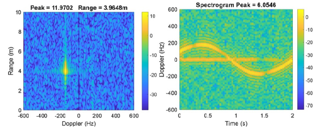
FIGURE 13 | HH-polarisation of a nano-drone response.
