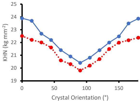
Figure 5. The variation in KHN with crystal orientation made using a 15g load at temperatures of 295K (blue solid line) and 323K (red dotted line).
