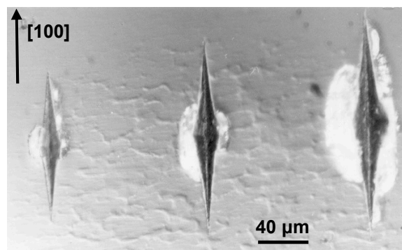
Figure 4. Knoop hardness impressions made using (from left to right) 15g, 25 and 35g loads. The longer diagonals of the indentations are aligned parallel to the [100] direction.
