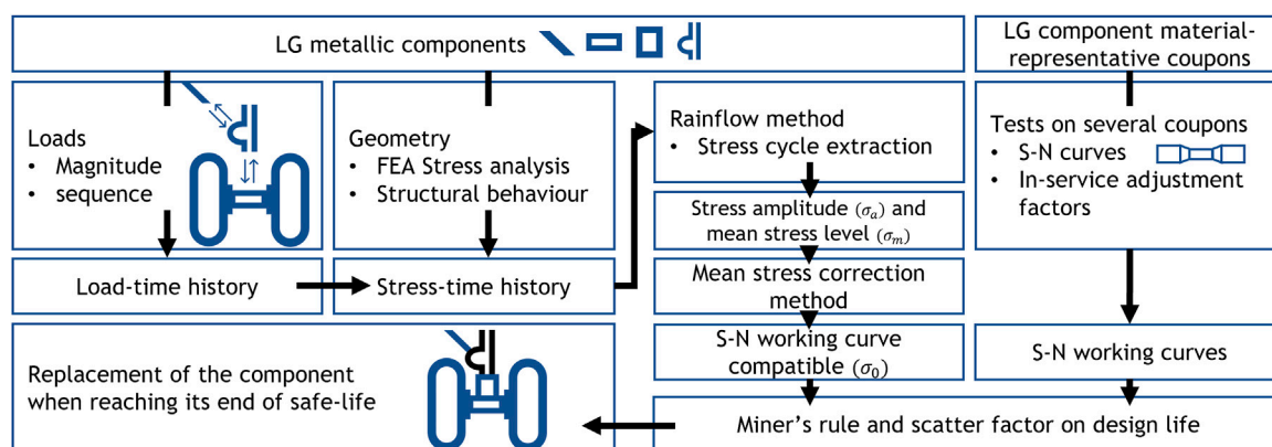
FIGURE 2 Steps for safe-life fatigue analysis of landing gear.
