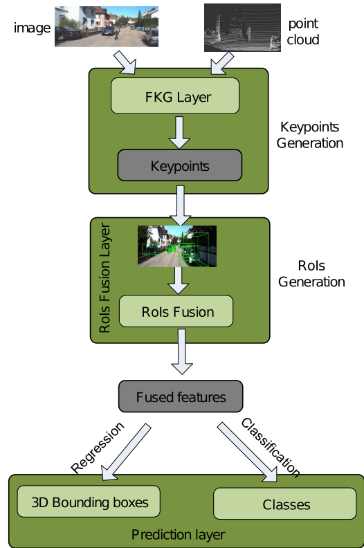
FIGURE 1. Flow chart of the proposed RoIFusion architecture. The flow chart consists of three main steps: keypoints generation, Rols generation, and 3D bounding boxes prediction. The FKG indicates keypoints generation layer.
