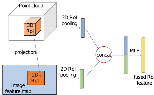
FIGURE 7. RoIs fusion layer.
