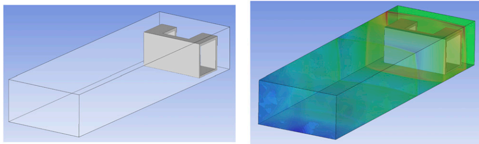
Figure 3. Autodyn, left image showing test structure and domain, right image showing simulation in progress. The domain size shown is 29.45 \times 9.5 \times 4.95 m (length \times width \times height).
