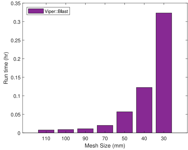
(b) Viper::Blast run times for 100kg simulation
