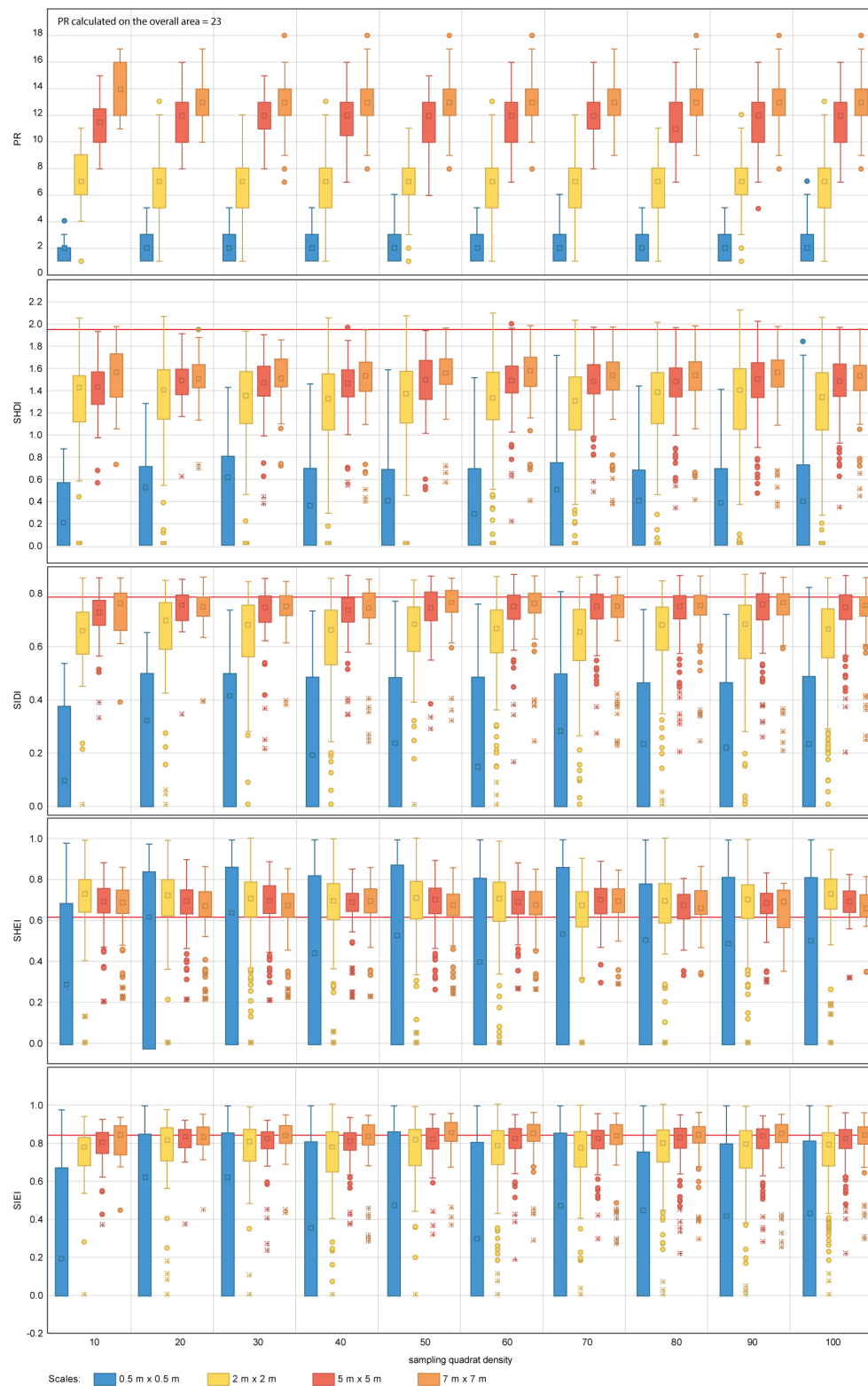
Figure 9. Diversity metric values obtained for the random sampling strategy for the range of scales and quadrat densities considered. The red horizontal line indicates the metric value obtained for the total area mapped. PR, SHDI, SIDI, SHEI and SIEI stand for Patch Richness, Shannon's Diversity Index, Simpson's Diversity index, Shannon's Evenness Index and Simpson's Evenness Index, respectively. The boxplots show the first, second (median), third and fourth quartiles. Circles and crosses indicate outliers and extreme values, respectively.
