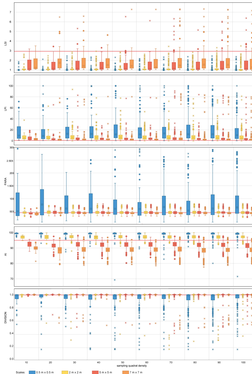
Figure 6. Area-density-edge, shape, contagion and interspersation metric values obtained for the nested sampling strategy for the range of scales and quadrat densities considered. The red horizontal line indicates the metric value obtained on the total area mapped. LSI, LPI, PARA, AI and DIVISION stand for Landscape Shape Index, Largest Patch Index, Perimeter Area Ratio Mean, Aggregation Index and Division Index, respectively. The boxplots show the first, second (median), third and fourth quartiles. Circles and crosses indicate outliers and extreme values, respectively.
