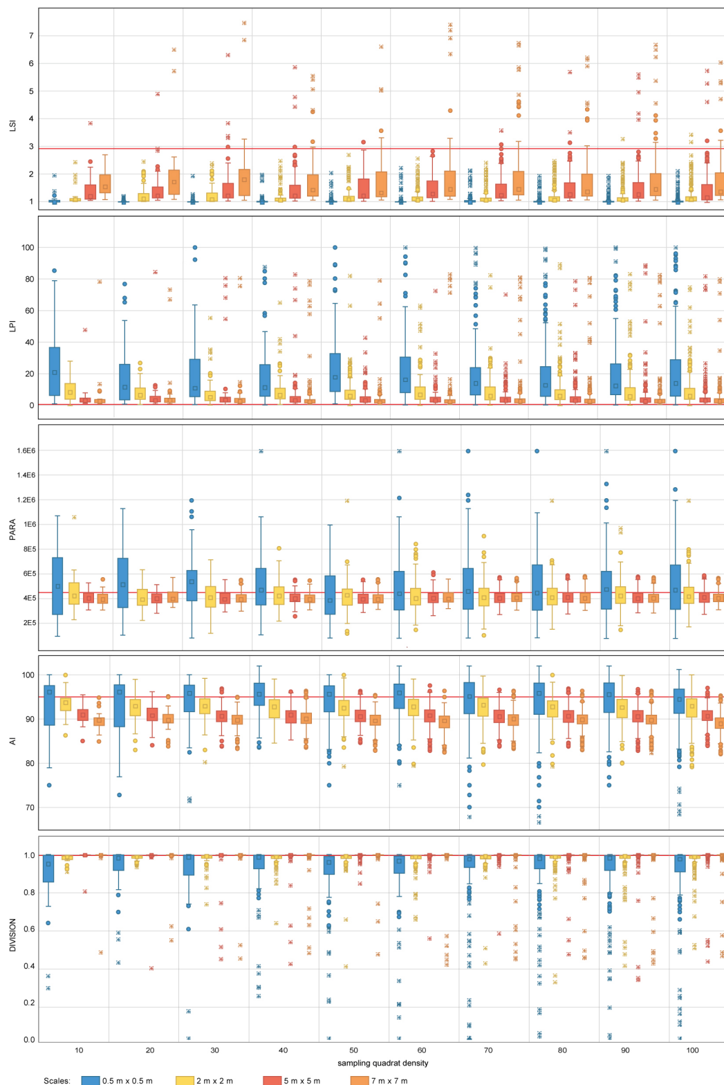
Figure 7. Area-density-edge, shape, contagion and interspersion metric values obtained for the random sampling strategy for the range of scales and quadrat densities considered. The red horizontal line indicates the metric value obtained on the total area mapped. LSI, LPI, PARA, AI and DIVISION stand for Landscape Shape Index, Largest Patch Index, Perimeter Area Ratio Mean, Aggregation Index and Division Index, respectively. The boxplots show the first, second (median), third and fourth quartiles. Circles and crosses indicate outliers and extreme values, respectively.
