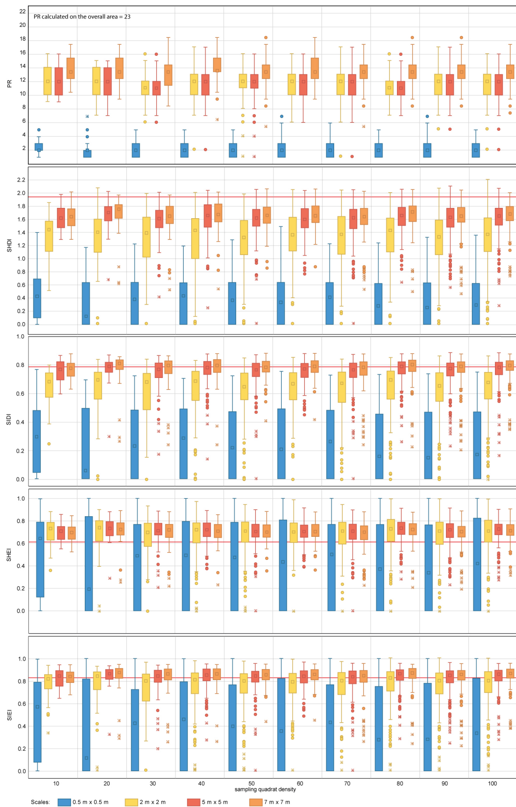
Figure 8. Diversity metric values obtained for the nested sampling strategy for the range of scales and quadrat densities considered. The red horizontal line indicates the metric value obtained for the total area mapped. PR, SHDI, SIDI, SHEI and SIEI stand for Patch Richness, Shannon's Diversity Index, Simpson's Diversity index, Shannon's Evenness Index and Simpson's Evenness Index, respectively. The boxplots show the first, second (median), third and fourth quartiles. Circles and crosses indicate outliers and extreme values, respectively.
