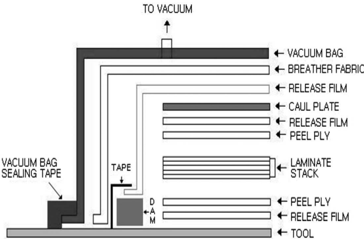
FIG. 2 Vacuum bagging process for graphite/epoxy composites.
