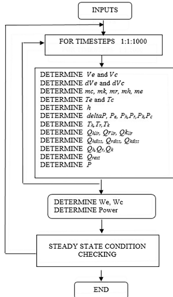
Fig. 5. Flow chart of the numerical simulation.
