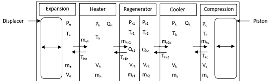
Fig. 4. The control volumes in the Stirling engine.
