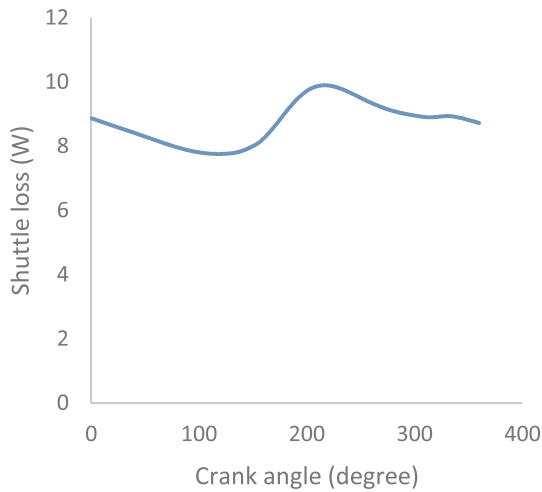
Fig. 9b. Shuttle loss in heat exchangers.
