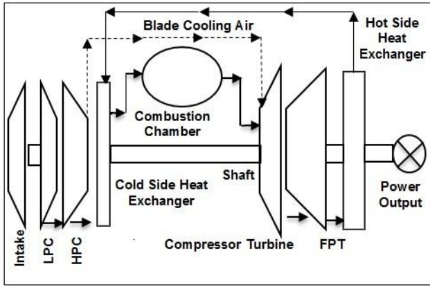
Figure 1: Schematic Layout of a two-spool Regenerated Turboshaft
