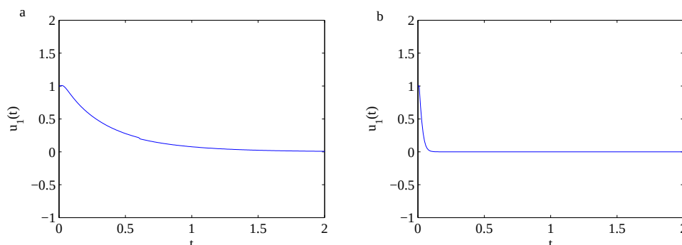
Figure 4. (a) Time sequence diagram of prey population u_1(t) when T = 2, \lambda_1 = 0.4 . (b) Time sequence diagram of predator population u_1(t) when T = 2, \lambda_1 = 0.1 .
