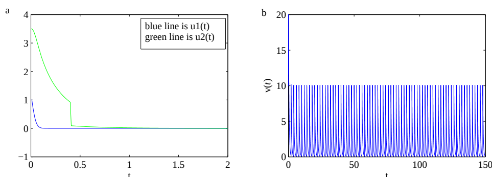
Figure 1. Dynamical behavior of system (1.1) with T = 2 . (a) Time sequence diagram of prey population u_1(t) and u_2(t) . (b) Time sequence diagram of predator population v(t) .
