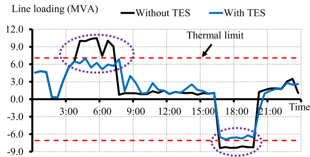
FIGURE 12. Power flow at head of the feeder (MVA) with procuring generation offers (4:00 a.m.-7:00 a.m.) and demand offers (4:30 p.m.-7:30 p.m.).
