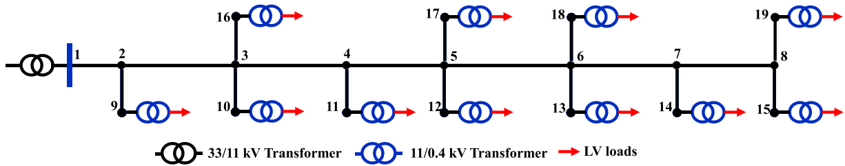
FIGURE 2. UKGDS 11 kV feeder.
