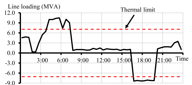
FIGURE 5. Power flow at head of the feeder (MVA) under dynamic residential pricing (before the functioning of TES).
