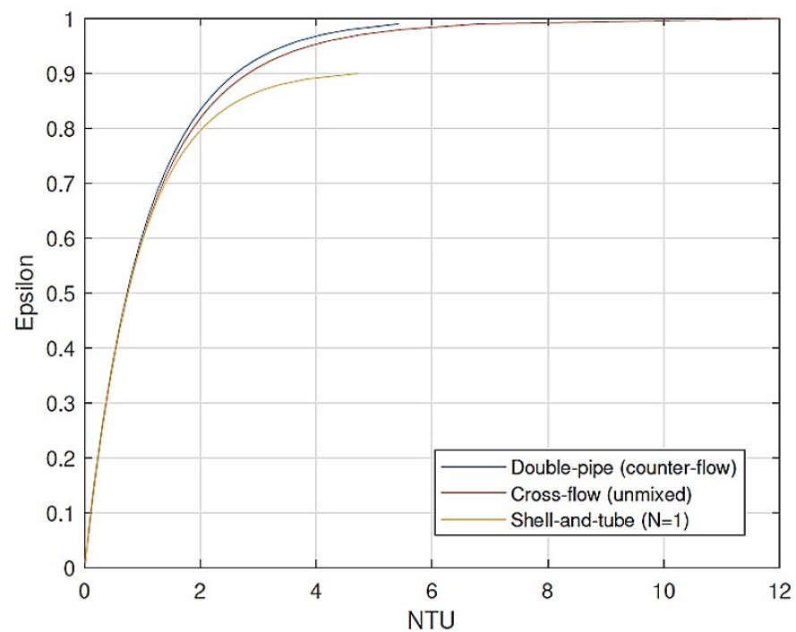
Figure 8. NTU vs. \varepsilon comparison for different types of heat exchangers.
